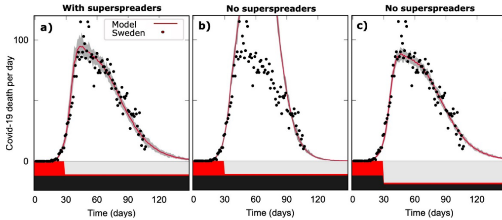
Figure 4. Model fit to daily COVID-19 fatalities in Sweden. Red lines shows average of 20 model runs; gray area is area into which 95% of trajectories fall. Best fit occurred when “other” contacts were reduced to 90% of normal (panel a). However, when superspreaders were removed from the model, those parameters no longer fit (panel b). Fit could be restored if “work/school” contacts were reduced to 40% of normal to achieve best fit while still reducing “other” contacts by 90%. The black and red stacked bar chart shows the proportion of “work/school” and “other” contacts allowed.
