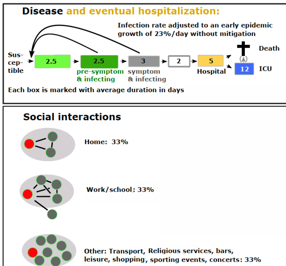
Figure 1: Schematic representation of our agent-based model. Agents progress in an SEIR framework, becoming infectious 2.5 days before symptom onset [12] (panel A). Most agents enter the recovered pool after 5 days with symptoms; some are hospitalized, and some of those enter the ICU or die according to conditional probabilities given in Table S1. The model's social network (panel B) allows contacts in three sectors, "Home", "Work/School" and "Other", with equal frequency.
