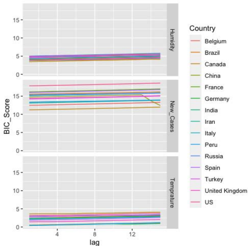
Supplementary Figure 1: lag optimization for Temperature, Humidity, New cases time series we calculated BIC score of AR (p) model at lag 1-15.
