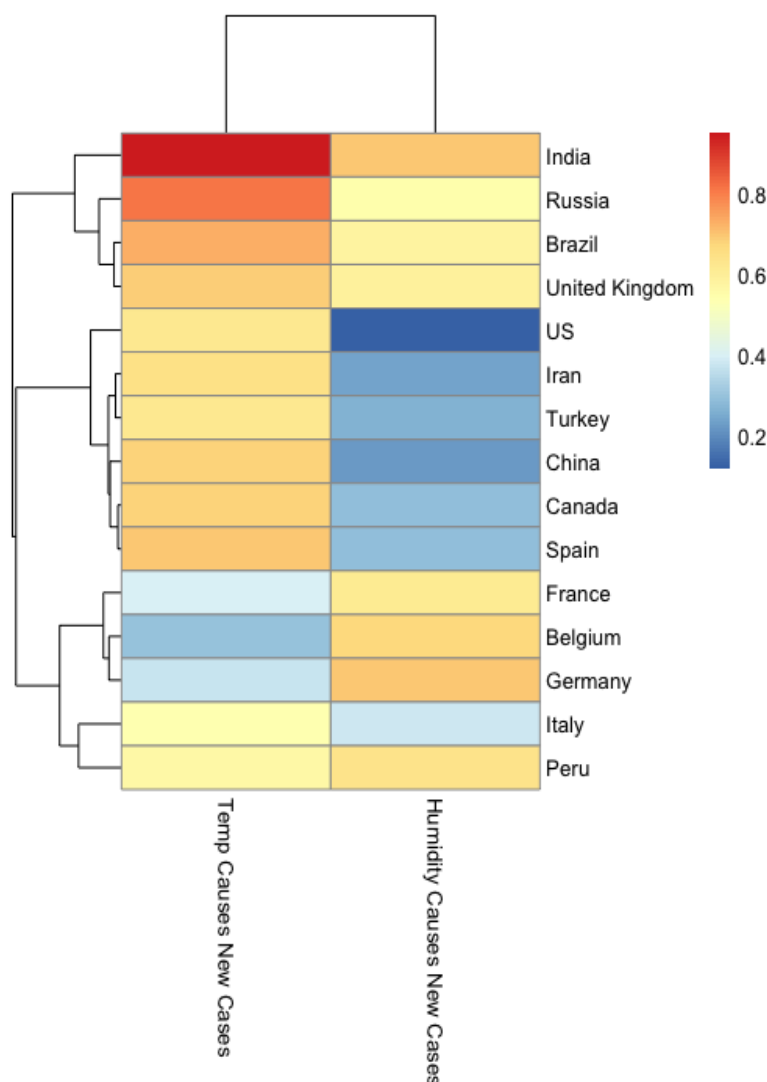
Figure2: Heatmap represents Pearson correlation between values generated by cross mapping of Temperature and Humidity state space to Infection State space and original value of infection.
