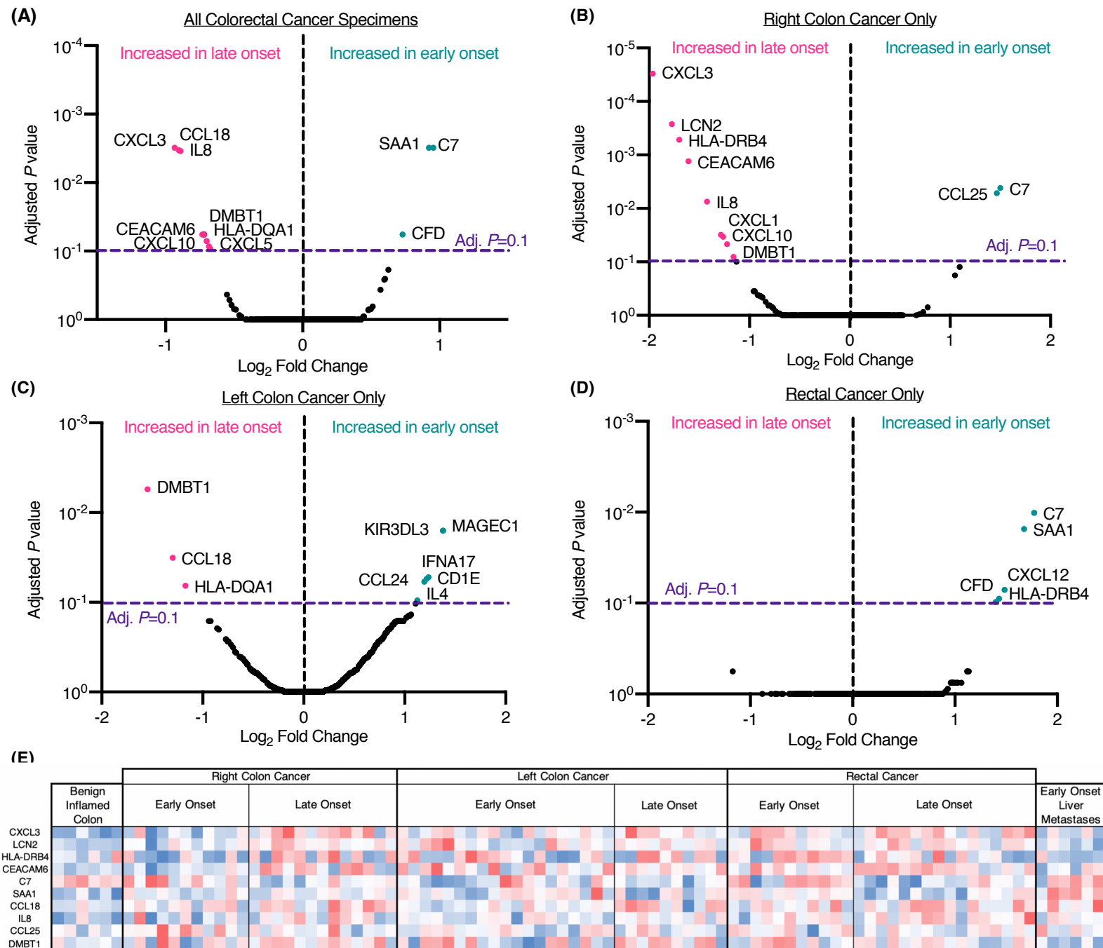
Figure 2: Immune microenvironment differences with age in colorectal cancer. Volcano plots depicts log 2 fold change in gene expression vs adjusted P-values of early vs late onset colorectal cancer patients. Nanostring Immune profiling panel (770 genes, human cancer immune panel) was used to generate expression profiles from RNA extracted from FFPE tissues slides. Raw counts were normalized to the best 10 housekeeping genes. The nSolver Advanced Analysis module was used to derive differential expression signatures according to Nanostring recommendations. Adjusted P-values were obtained with a Benjamini-Hochberg post-hoc correction. (A) Early (N=40) vs late onset (N=39) in all colorectal cancer specimens. (B) Right colon cancer specimens only (early N=10, late N=14). (C) Left colon cancer specimens only (early N=19, late N=10). (D) Rectal cancer specimens only (early N=11, late N=15). (E) Heatmap of the top 10 most differentially expressed immune genes with blue representing low relative gene expression and red representing high relative gene expression compared to other specimens.
