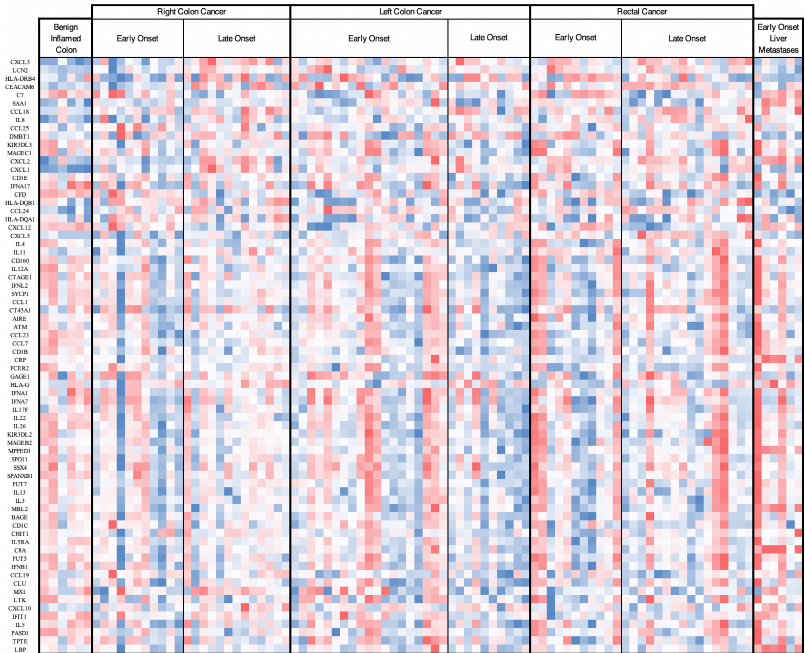
Supplemental Figure 1: Heatmap of differentially expressed immune genes between early and late onset colorectal cancer. Nanostring Immune profiling panel (770 genes, human immune panel) was used to generate expression profiles from RNA extracted from FFPE tissues slides. Raw counts were normalized to the best 10 housekeeping genes. The nSolver Advanced Analysis module was used to derive differential expression signatures according to Nanostring recommendations. Adjusted P-values were obtained with a Benjamini-Hochberg post-hoc correction. Genes with an adjusted p value >0.2 in all colorectal cancer, right colon cancer, left colon cancer, and rectal cancer specimens are included in the heatmap. The genes are ordered by p values with lowest p values at the top. Blue represents low relative gene expression and red represents high relative gene expression compared to other specimens.
