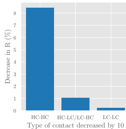
Figure 7: The effect of reducing each contact mode by 10% under the simple compartmental model presented here.
