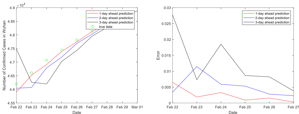
(a) Average number of predictions (b) Relative prediction error
