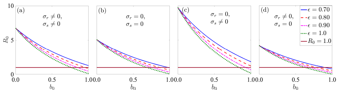
Figure 7: Numerical simulations of the basic reproduction number R_0 , against ITN coverage b_0 , illustrating insecticide-impregnated bed-net coverage levels required for bringing malaria under control for four values of insecticide-impregnated bed-net efficacy ( \epsilon ) when mosquito resistant to insecticides is permanent or non-permanent. (a) Mosquito resistance to insecticides is not permanent and acquired through mosquito resistant and through transition of mosquitoes occurring at rate \sigma_s \neq 0 . (b) Mosquito resistance is permanent and is only acquired through mosquito recruitment. (c) Resistance is permanent and acquired through mosquito recruitment and adult sensitive mosquito transition. (d) Resistance is not permanent and is acquired only through mosquito-recruitment. Other parameters used for the simulations are presented in Table 1.
