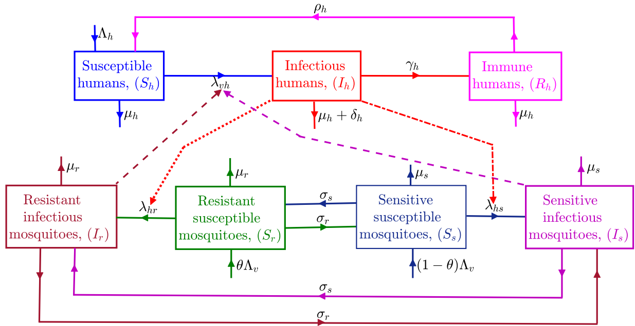
Figure 1: Model flow-chart showing the flow of humans and mosquitoes between different classes that represent the status of the disease (solid lines) and interactions between humans and mosquitoes (non solid lines). Interactions resulting in sensitive and resistant susceptible mosquito infections by infectious humans are denoted by dash-dotted and dotted lines, respectively, and interactions resulting in susceptible human infections by sensitive and resistant infectious mosquitoes are denoted by dark red and light magenta dashed lines, respectively. The human population is broken down into susceptible S_h , infectious I_h , and partially immune R_h , while the mosquito population comprises susceptible sensitive and resistant ( S_s and S_r , respectively,) and infectious sensitive and resistant classes ( I_s and I_r , respectively). Descriptions of the transition rates (parameters) are presented in the text and in Table 1, while the forces of infection \lambda_{vh} , \lambda_{hs} and \lambda_{hr} are described in the text and presented in Eq. (2.6).
