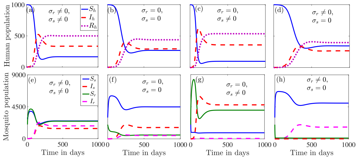
Figure 3: Numerical simulation results illustrating the existence of an endemic equilibrium to System (2) when R_0 > 1 . Graphs (a) and (e) show the dynamics for the case in which resistance is acquired at rate \sigma_s \neq 0 and lost over time at rate \sigma_r \neq 0 . Graphs (b) and (f) illustrate the dynamics when resistance is acquired only through mosquito recruitment and is permanent. Graphs (c) and (g) illustrate the dynamical behavior of the system when resistance is permanent and can be acquired through mosquito recruitment or transition of sensitive mosquitoes to resistant mosquitoes at rate \sigma_s \neq 0 . Graphs (d) and (h) illustrate the dynamical behavior of the system when resistance is not permanent and can only be acquired through mosquito recruitment, i.e., \sigma_r \neq 0 and \sigma_s = 0 . Parameter values used for the simulations are presented in Table 1.
