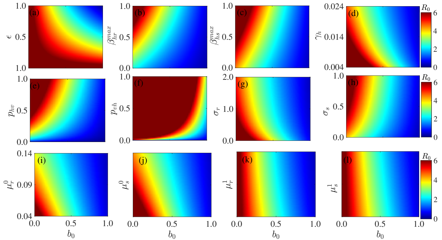
Figure 9: Heat maps from numerical simulations illustrating the impact on the basic reproduction number R_0 , of ITN coverage b_0 and (a) ITN efficacy \epsilon , (b) the maximum biting rate of resistant mosquitoes \beta_{hr}^{max} , (c) the maximum biting rate of sensitive mosquitoes \beta_{hs}^{max} , (d) the recovery rate from infection \gamma_h , (e) the probability of an infectious human infecting a susceptible mosquito p_{hv} , (f) the probability of infectious mosquito infecting a susceptible human p_{vh} , (g) the rate at which resistant mosquitoes lose resistance \sigma_r , (h) the rate at which sensitive mosquitoes develop resistance \sigma_s , (i) the natural mortality rate of resistant mosquitoes \mu_r^0 , (j) the natural mortality rate of sensitive mosquitoes \mu_s^0 , (k) the ITN-induced mortality rate of resistant mosquitoes \mu_r^1 , and (l) the ITN-induced mortality rate of sensitive mosquitoes \mu_s^1 . The values of the other parameters are presented in Table 1.
