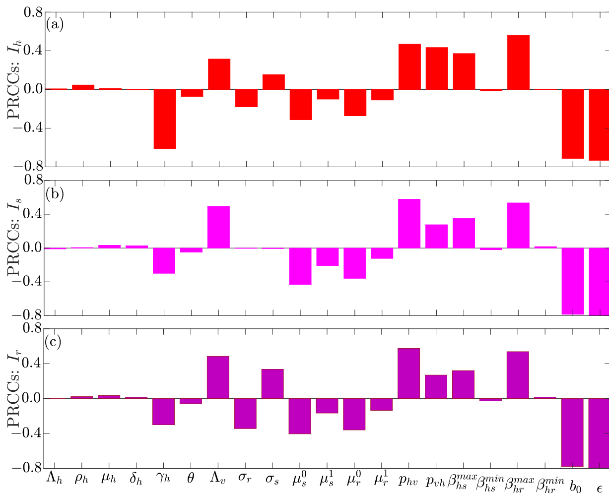
Figure 6: Global uncertainty and sensitivity analysis results showing the contributions of uncertainty or variability in model parameters to uncertainty or variability to the (a) infectious human population ( I_h ), (b) sensitive mosquito population ( I_s ), and (c) resistant mosquito population ( I_r ). Positive PRCCs represent positive correlations, i.e., an increase in a parameter will trigger an increase in I_h , I_s , or I_r , while negative PRCCs represent negative correlations. The magnitude of the PRCC represents the strength or level of significance. Parameters used for the simulations are presented in Table 1.
