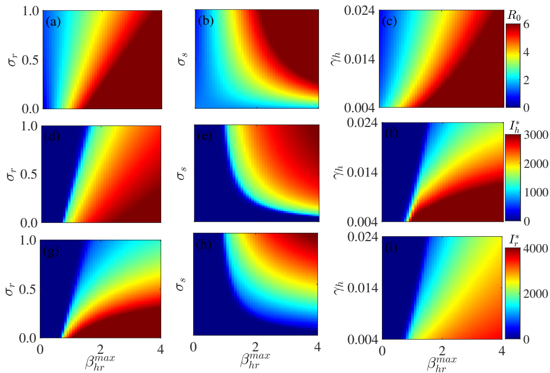
Figure 11: Numerical simulation results illustrating the effects on the basic reproduction number ((a)-(c)), the infectious human population ((d)-(f)), and the resistant infectious mosquito population ((g)-(i)) for combinations of the maximum biting rate of resistant mosquitoes \beta_{hr}^{max} the rate at which resistance is lost, \sigma_r ((a), (d), (g)), and the development rate of resistance, \sigma_r ((b), (e), (h)), and the human recovery rate, \sigma_r ((c), (f), (i)). The other parameter values used for the simulations are presented in Table 1.
