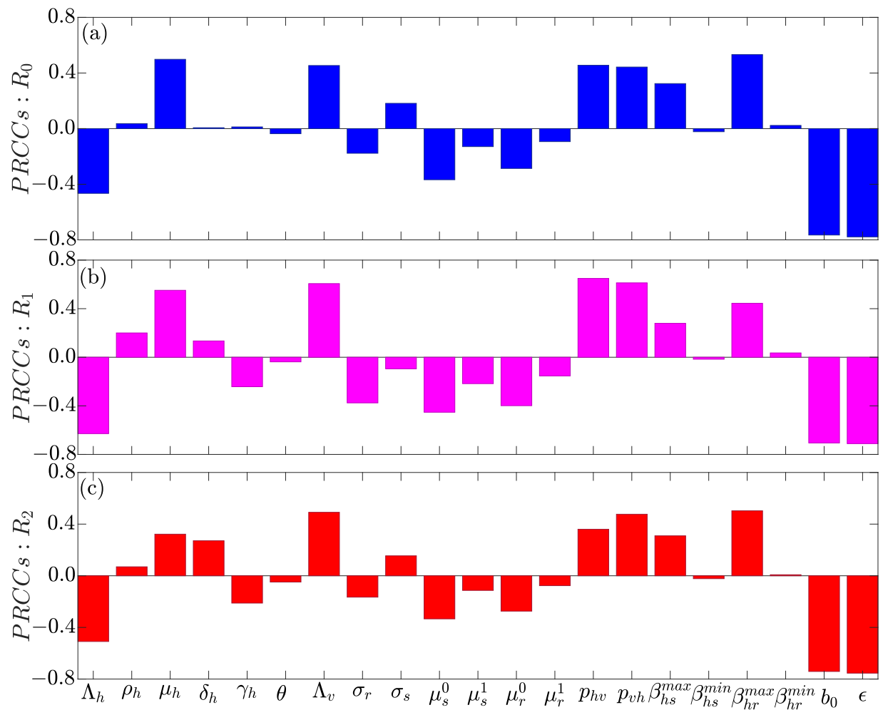
Figure 5: Global uncertainty and sensitivity analysis results showing the contributions of uncertainty or variability in model parameters to uncertainty or variability to the (a) basic reproduction number R_0 , and (b)-(c) threshold quantities R_1 and R_2 (Eq. (3.7)). Positive PRCCs represent positive correlation, i.e., an increase in a parameter will trigger an increase in R_0 , R_1 , or R_2 , while negative PRCCs represent negative correlations. The magnitude of the PRCC represents the level of significance. Parameters used for the simulations are presented in Table 1.
