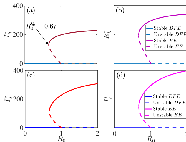
Figure 4: Bifurcation plot of the equilibrium infectious humans, I_h^* ((a)), partially immune humans, R_h^* ((b)) sensitive infectious mosquitoes, I_s^* ((c)), and the resistant infectious mosquitoes, I_r^* ((d)) against the basic reproduction number, R_0 . Model (2) exhibits a backward bifurcation for R_0^{bb} \leq R_0 < 1 ( R_0^{bb} = 0.67 ), where an unstable endemic equilibrium (EE) is located between a stable endemic equilibrium (EE) and a stable disease free equilibrium (DFE). The ITN coverage ( b_0 ) is varied, while the other parameter values are as given in Table 1.
