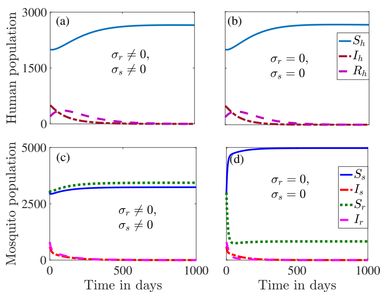
Figure 2: Numerical simulation results illustrating the existence of a disease free equilibrium to System (2) when R_0 < 1 . Graphs (a) and (c) show the dynamics for the case in which resistance is acquired at rate \sigma_s \neq 0 and lost over time at rate \sigma_r \neq 0 . Graphs (b) and (d) illustrate the dynamics when resistance is acquired only through mosquito recruitment and is permanent. Parameter values used for the simulations are presented in Table 1.
