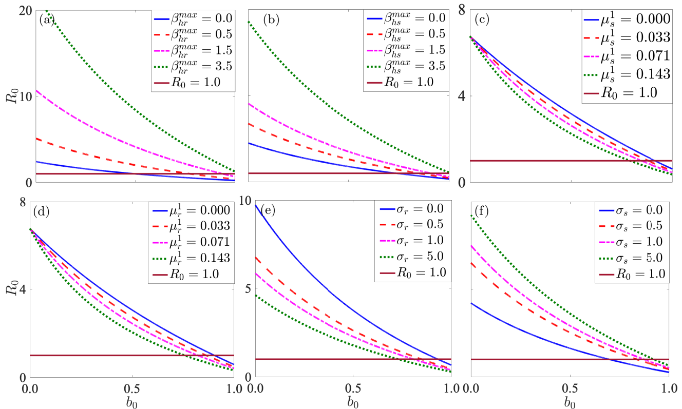
Figure 8: Numerical simulation results of the basic reproduction number R_0 , against ITN coverage b_0 , illustrating various insecticide-impregnated bed-net coverage levels required for bringing malaria under control for four values of (a)-(b) the maximum biting rates of resistant and sensitive mosquitoes ( \beta_{hr}^{max} and \beta_{hs}^{max} , respectively), (c)-(d) insecticide-induced mortality rates of resistant and sensitive mosquitoes ( \mu_r^1 and \mu_s^1 ), and (e)-(f) the resistant development and loss rates for mosquitoes ( \sigma_r and \sigma_s , respectively). Other parameters used for the simulations are presented in Table 1.
