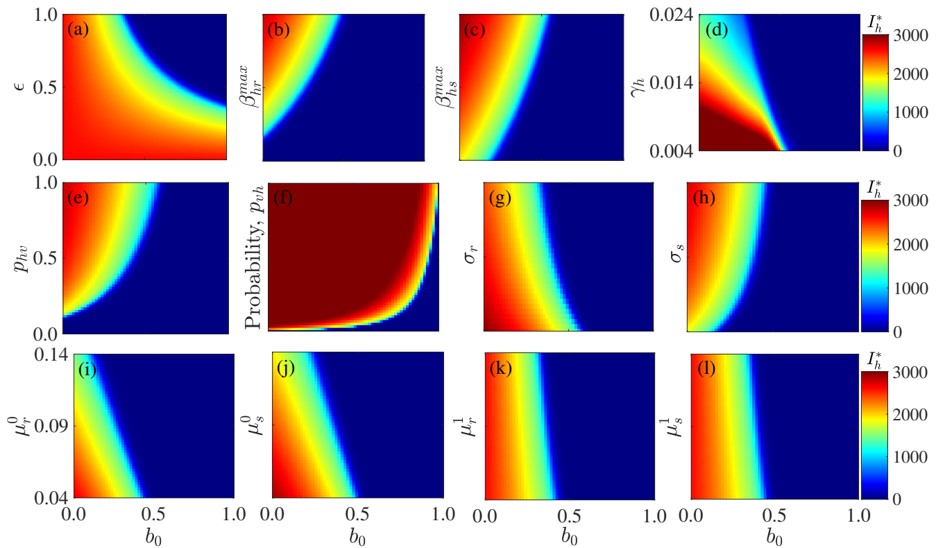
Figure 10: Numerical simulation results illustrating the impact on the Infectious human population I_h , of ITN coverage b_0 and (a) ITN efficacy \epsilon , (b) the maximum biting rate of resistant mosquitoes \beta_{hr}^{max} , (c) the maximum biting rate of sensitive mosquitoes \beta_{hs}^{max} , (d) the recovery rate from infection \gamma_h , (e) the probability of an infectious human infecting a susceptible mosquito p_{hv} , (f) the probability of infectious mosquito infecting a susceptible human p_{vh} , (g) the rate at which resistant mosquitoes lose resistance \sigma_r , (h) the rate at which sensitive mosquitoes develop resistance \sigma_s , (i) the natural mortality rate of resistant mosquitoes \mu_r^0 , (j) the natural mortality rate of sensitive mosquitoes \mu_s^0 , (k) the ITN-induced mortality rate of resistant mosquitoes \mu_r^1 , and (l) the ITN-induced mortality rate of sensitive mosquitoes \mu_s^1 . Other parameters used for the simulations are presented in Table 1.
