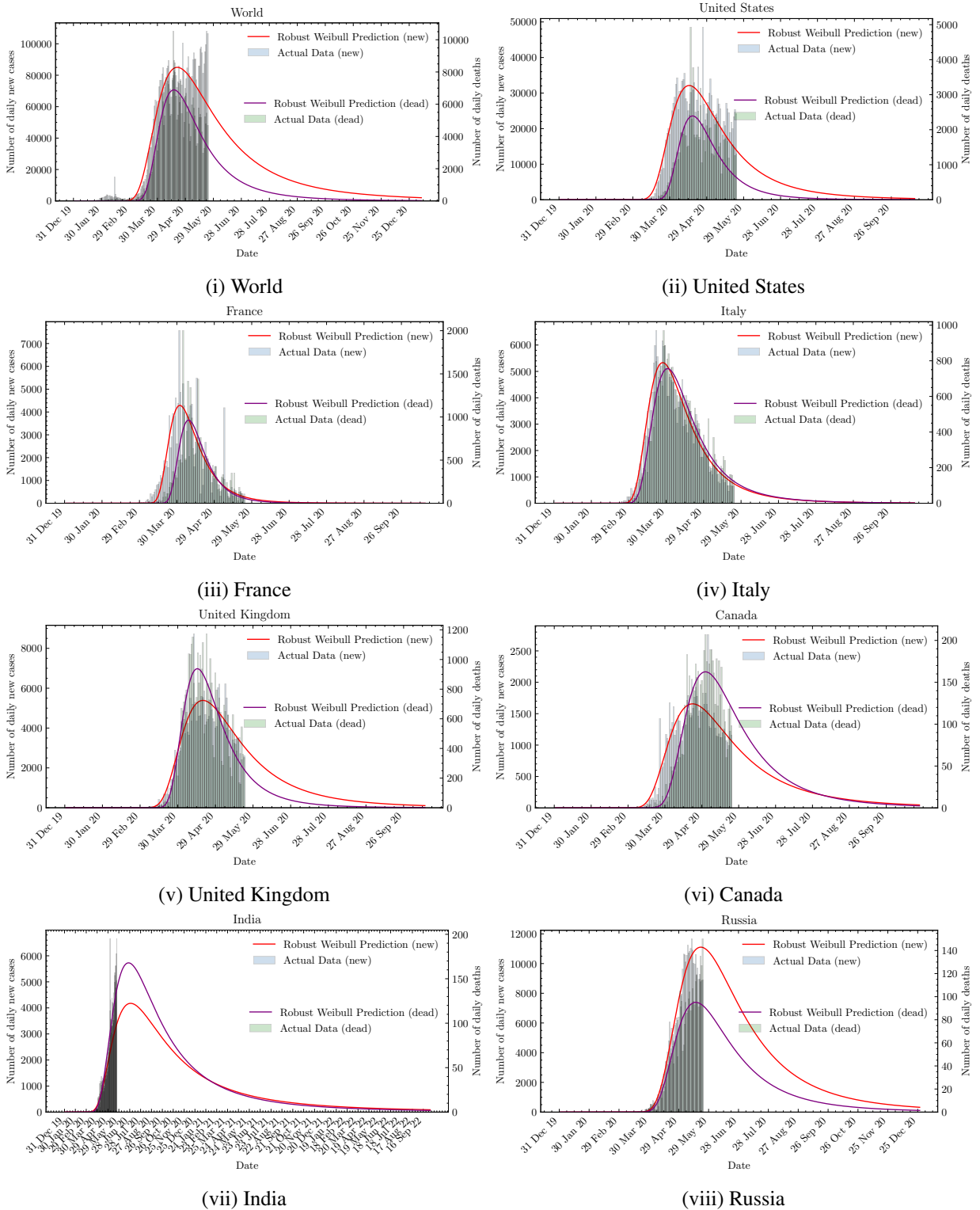
Figure 2: New daily cases and deaths curves for world and a few of the highest affected countries
