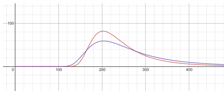
Figure 3: Death cases for constant k = 10000 and \gamma = 2500 with (a) higher values of \alpha = 38.5 , \beta = 4.6 in red and (b) lower values of \alpha = 22 , \beta = 3.4 in purple.
