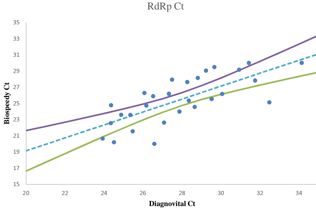
Figure 2. The Deming regression of Ct values obtained for RdRp gene for the two separate kits and 95% confidence interval for the regression line. Any data pair with any negative results are omitted.
