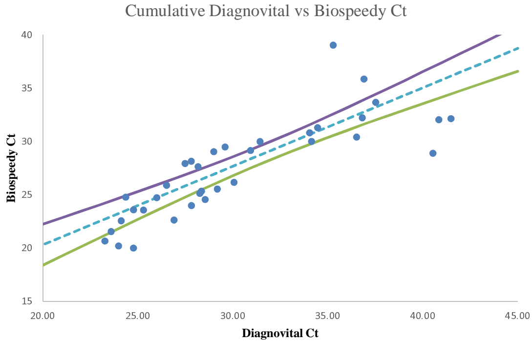
Figure 4. The Deming regression of the cumulative Ct values of Diagnostical and RdRp Ct values of Biospeedy and 95% confidence interval for the regression line. The cumulative Ct values were calculated by the sum of arbitrary copy numbers of gene E and RdRp genes obtained through 2^{-Ct} . The arbitrary copy numbers for negatives were assumed as zero.
