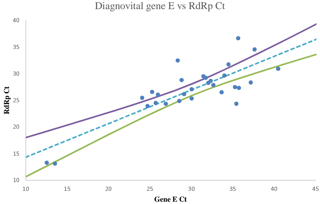
Figure 3. The Deming regression of Ct values obtained for RdRp gene and gene E for Diagnovital and 95% confidence interval for the regression line. Any data pair with any negative results are omitted.
