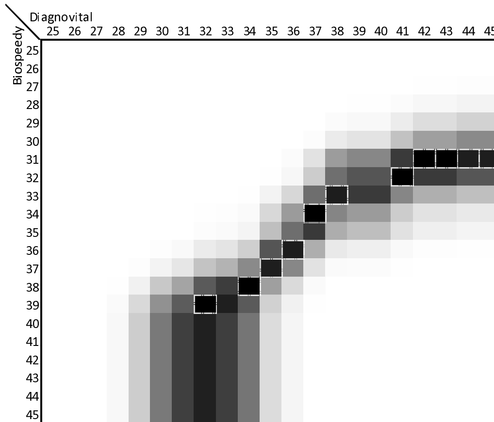
Figure 5. Heat map for chi-square scores obtained for a range of thresholds for Biospeedy and Diagnovital kits. Black and white squares indicate chi-square score of 1 and 0, respectively. The black squares with white borders indicate Ct threshold combinations where chi square scores are above 0.88.
