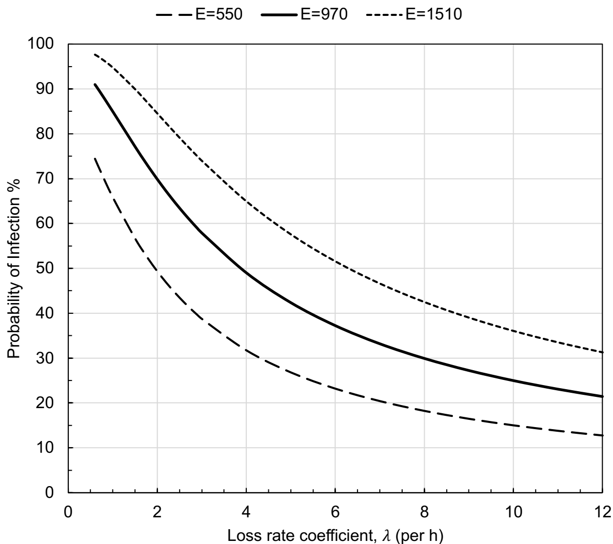
Figure 1. Probability of infection for each rehearsal participant as a function of loss rates for varying airborne quanta emission rates ( E , q h^{-1} ). Infection probability is plotted for the predicted mean emission rate ( 970 q h^{-1} ) and the 10 th and 90 th percentile emission rates ( 550 and 1510 q h^{-1} , respectively.) A rehearsal duration of 2.5 hours, an indoor volume of 810 m^3 and a volumetric breathing rate of 1.0 m^3 h^{-1} were assumed.
