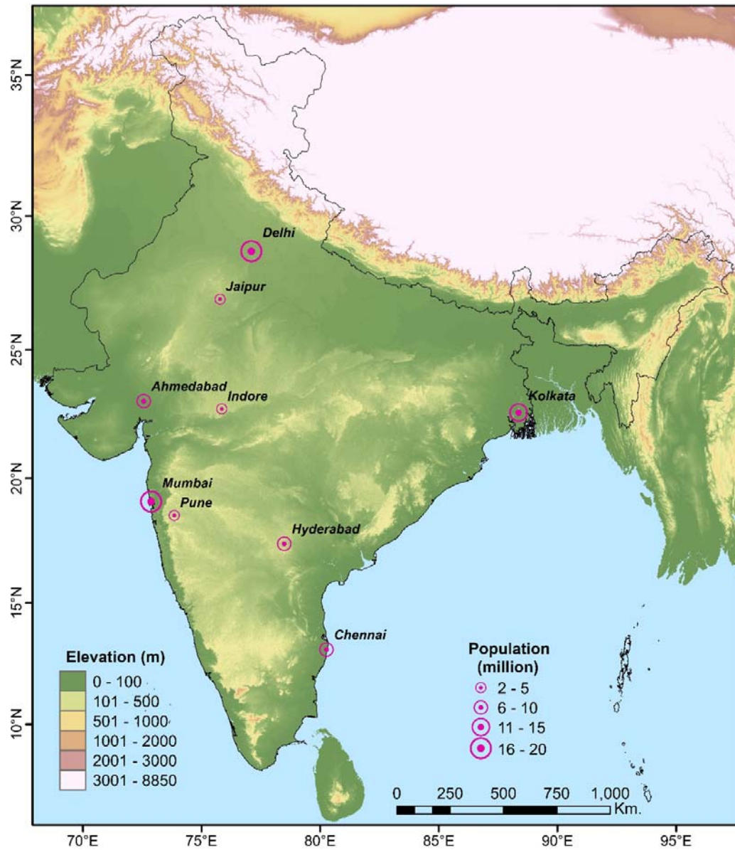
480 Fig. 1 Location of the selected cities in India along with the total population of those cities.
