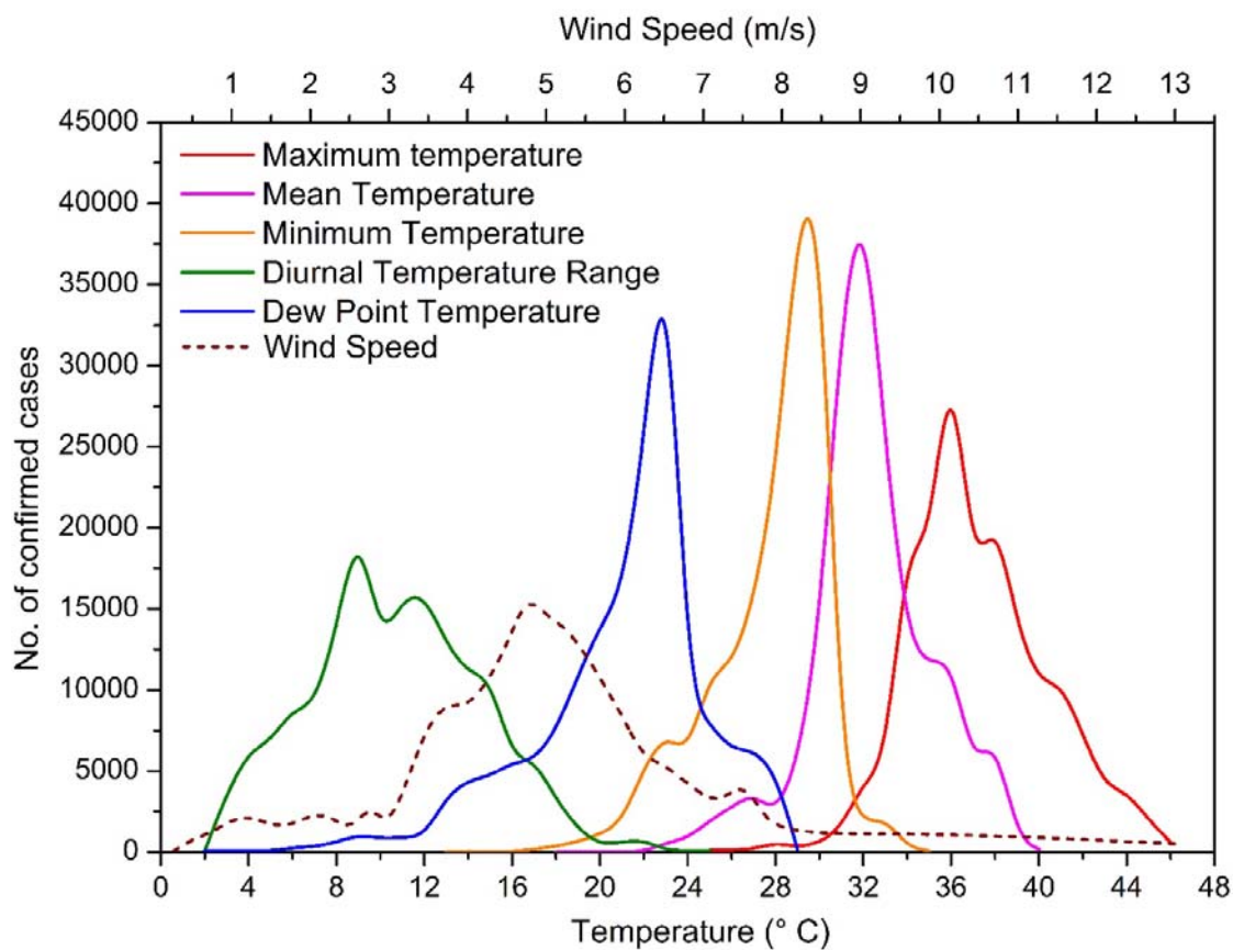
513 Fig. 5 Influence of weather parameters on count of confirmed cases with a lag of 12-16 days.
