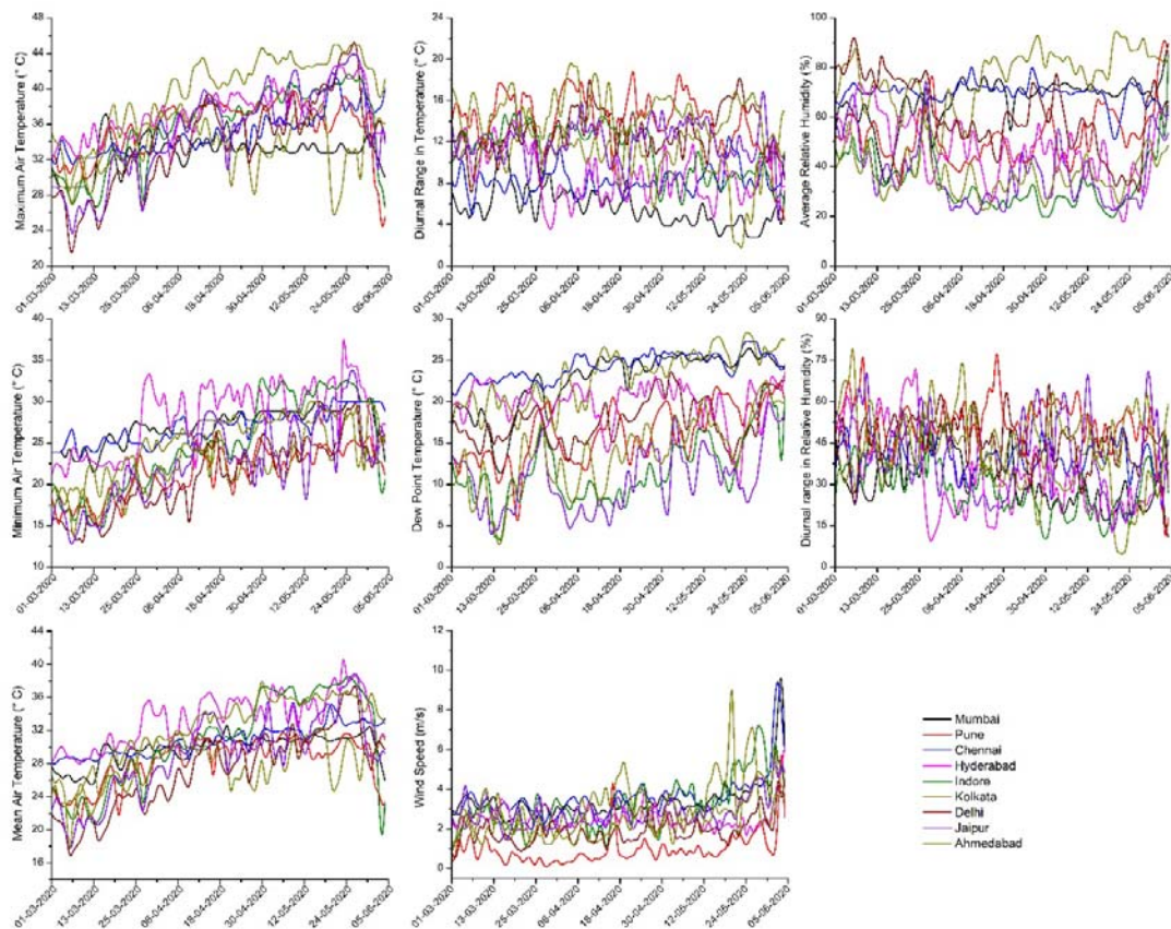
492 Fig. 3 Pattern of Daily Weather over the selected cities in India.
