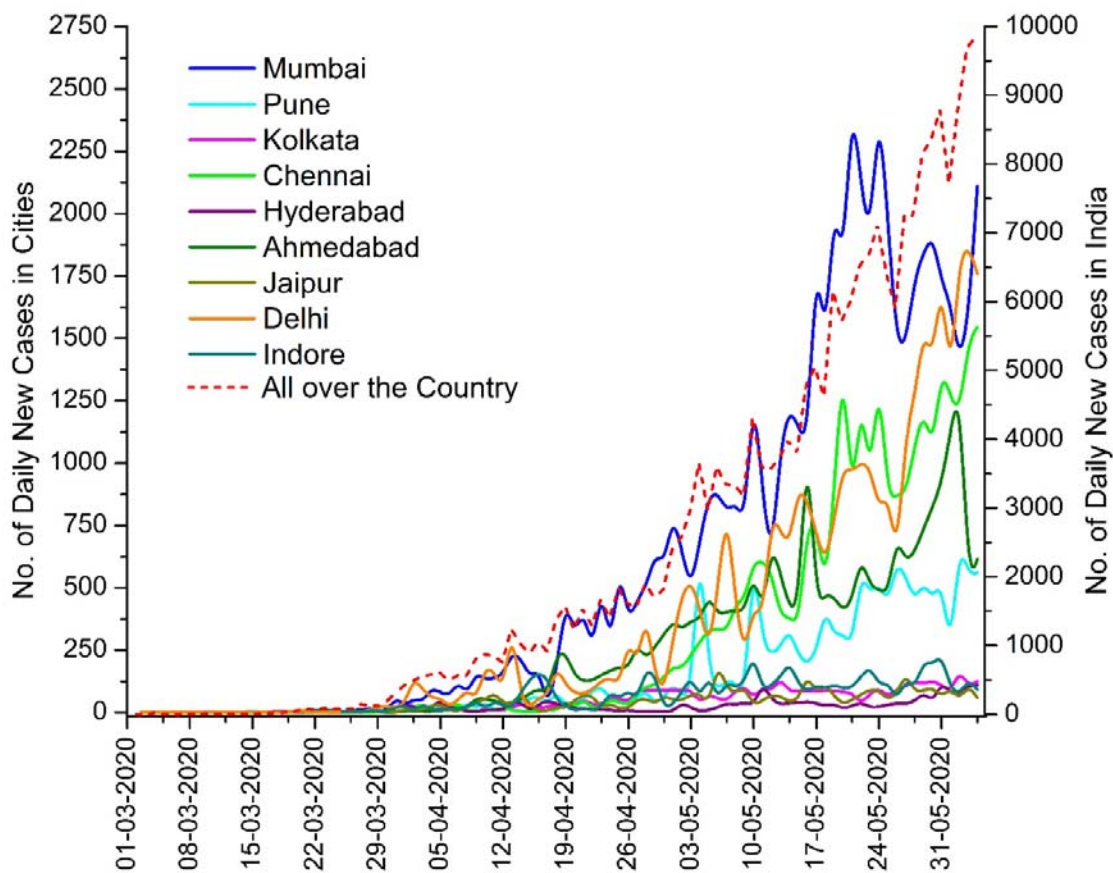
488 Fig. 2 Trend of daily confirmed cases over selected cities and all-over the country.
