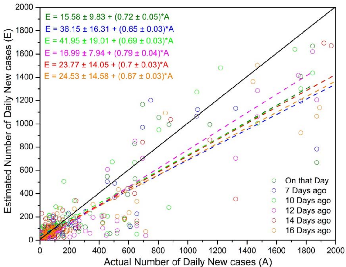
503 Fig. 4 Validation of SVM based regression model for estimating daily transmission.
