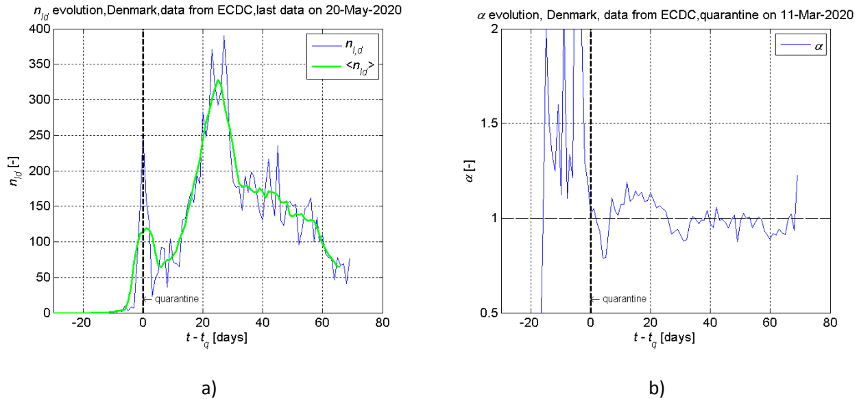
Figure 14. Dynamics of the daily new cases n_{I,d} (a) and the growth rate of new cases \alpha (b) for Denmark. Vertical black line points the day of imposed quarantine on 2020 March 11. Data collected from [2].
