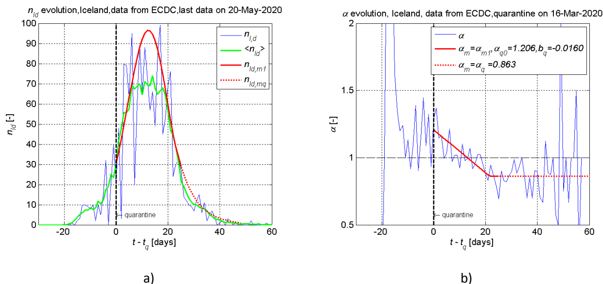
Figure 8. Dynamics of the daily new cases n_{id} (a) and the growth rate of new cases \alpha (b) for Iceland. Vertical black line points the day of imposed quarantine on 2020 March 16. Data collected from [2].
