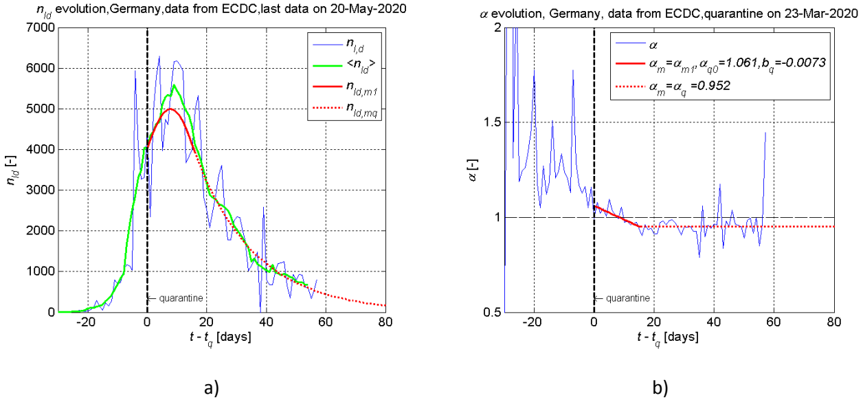
Figure 12. Dynamics of the daily new cases n_{I,d} (a) and the growth rate of new cases \alpha (b) for Germany. Vertical black line points the day of imposed quarantine on 2020 March 23. Data collected from [2].
