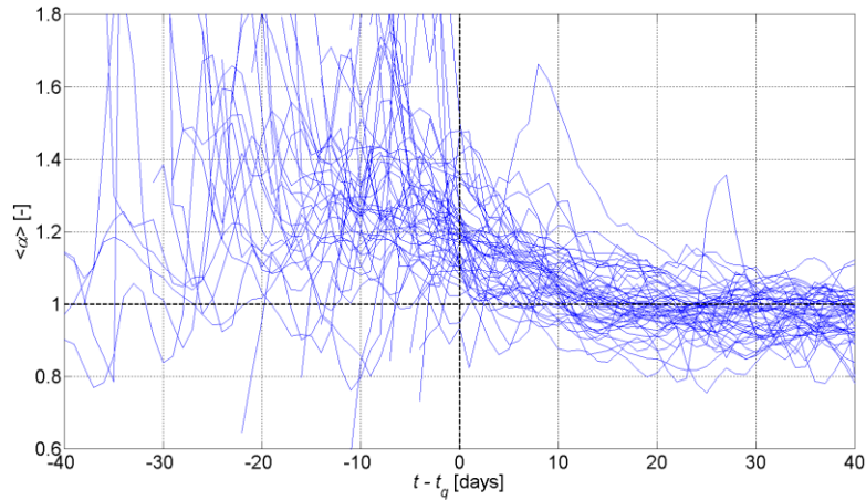
Figure 4. The averaged growth rate of new infection cases \langle \alpha \rangle versus time for 46 countries. Vertical black line points the day of imposed quarantine.
