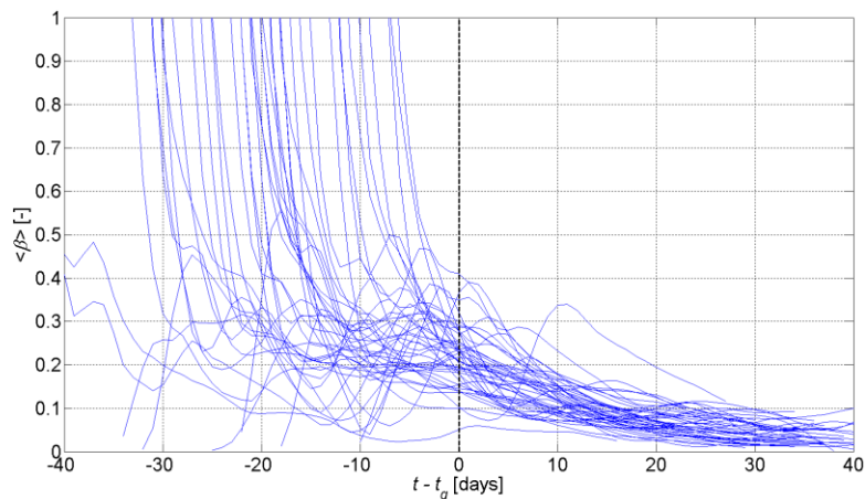
Figure 1. The averaged infectious rate \langle \beta \rangle versus time for 46 countries. Vertical black line points the day of imposed quarantine.
