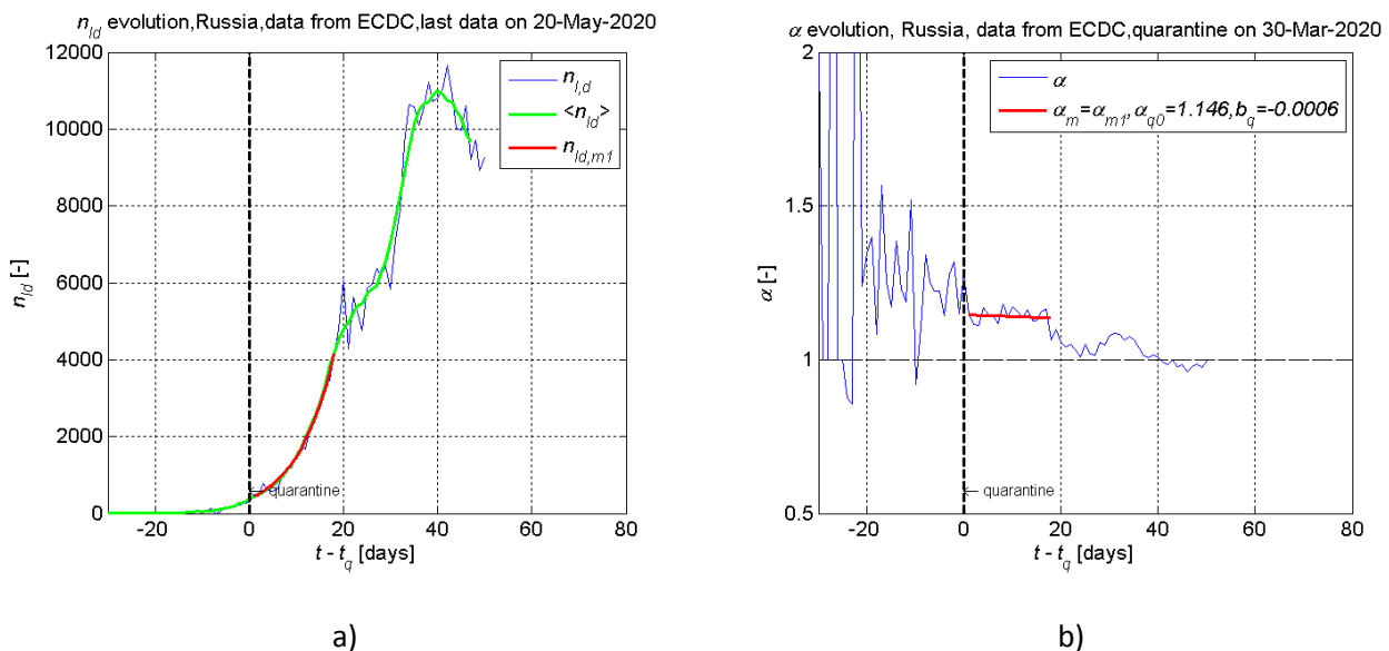
Figure 15. Dynamics of the daily new cases n_{I,d} (a) and the growth rate of new cases \alpha (b) for Russia. Vertical black line points the day of imposed quarantine on 2020 March 30. Data collected from [2].
