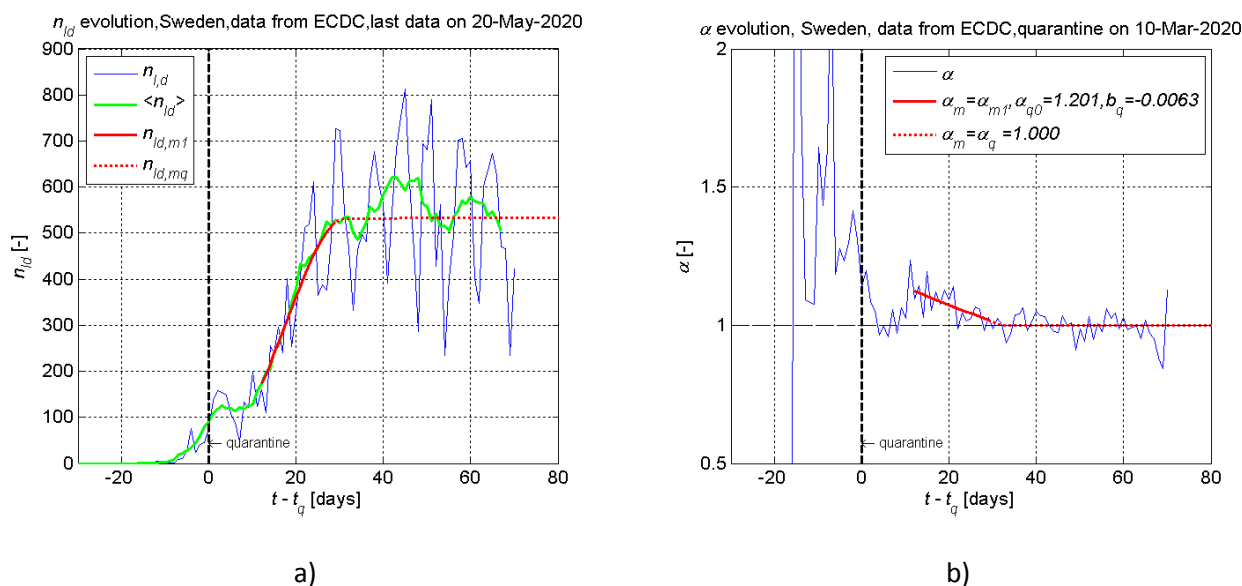
Figure 17. Dynamics of the daily new cases n_{i,d} (a) and the growth rate of new cases \alpha (b) for Sweden. Vertical black line points the day of imposed initial quarantine actions on 2020 March 10. Data collected from [2].
