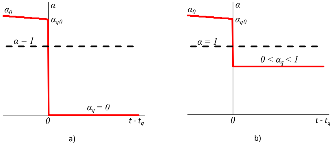
Figure 2. Idealized scenario of the growth rate of new cases \alpha dynamics with quarantine effectiveness e_q : a) e_q = 1 , b) e_q < 1 .
