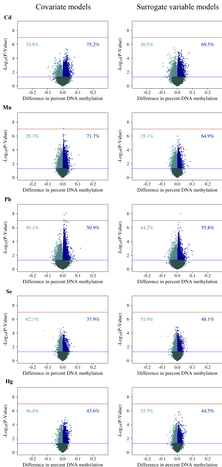
Figure 1. Volcano plots of global trends in methylation in covariate models 1 and surrogate variable models 2 for each trace metal. Row 1 includes plots for cadmium (Cd), row 2 includes plots for manganese (Mn), row 3 includes plots for lead (Pb), row 4 includes plots for selenium (Se), and row 5 includes plots for total mercury (Hg). Column 1 includes plots for covariate models, and column 2 includes plots for surrogate variable models. (n=97 samples; n= 348,438 probes)
