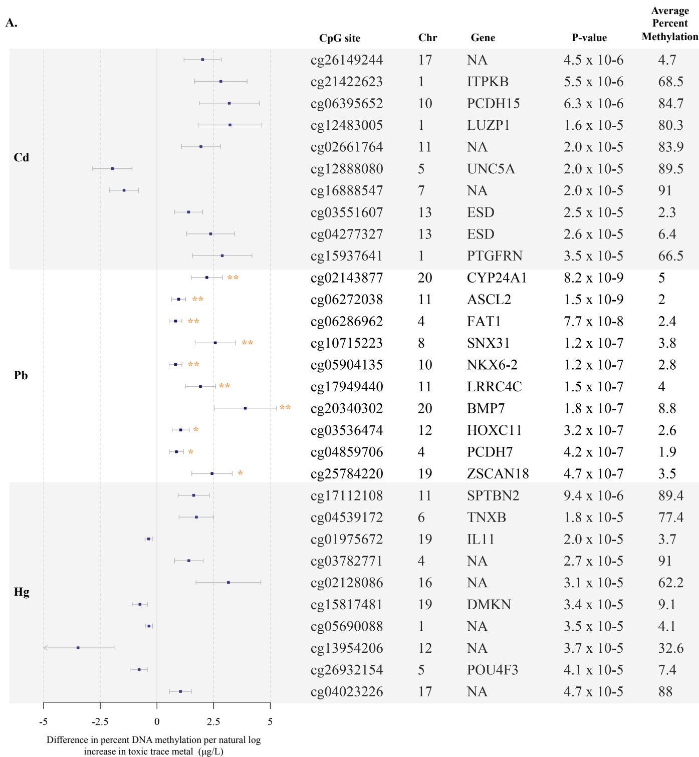
Figure 2. Top 10 CpG sites associated with blood trace metals from regression models adjusted for cell type principal components 1 and 2, maternal age, fetal sex, and hybridization date (n=97 samples). Figure 2A reports associations with cadmium (Cd), lead (Pb), and total mercury (Hg). Figure 2B reports associations with manganese (Mn), selenium (Se).
