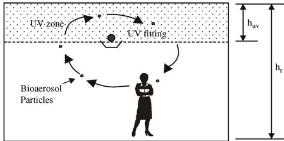
Figure 1. An upper-room UVGI installation.
