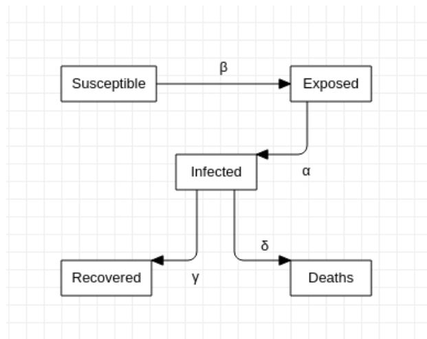
Fig. 3: SEIRD Model
