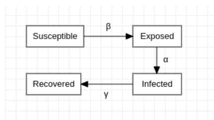
Fig. 2: SEIR Model
