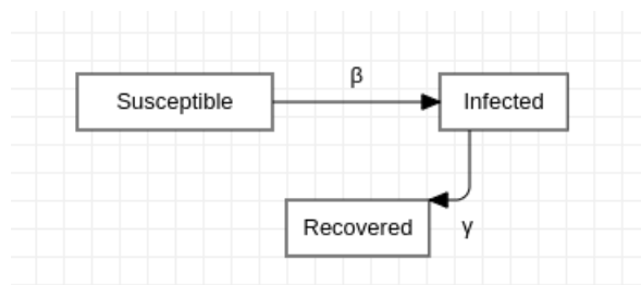
Fig. 1: SIR Model
