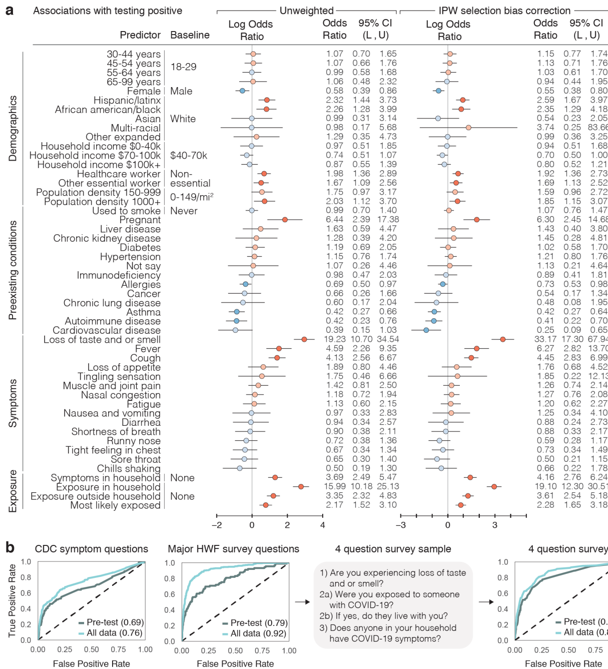
Figure 3: SARS-CoV-2 PCR Test Result Associations and Predictions.
