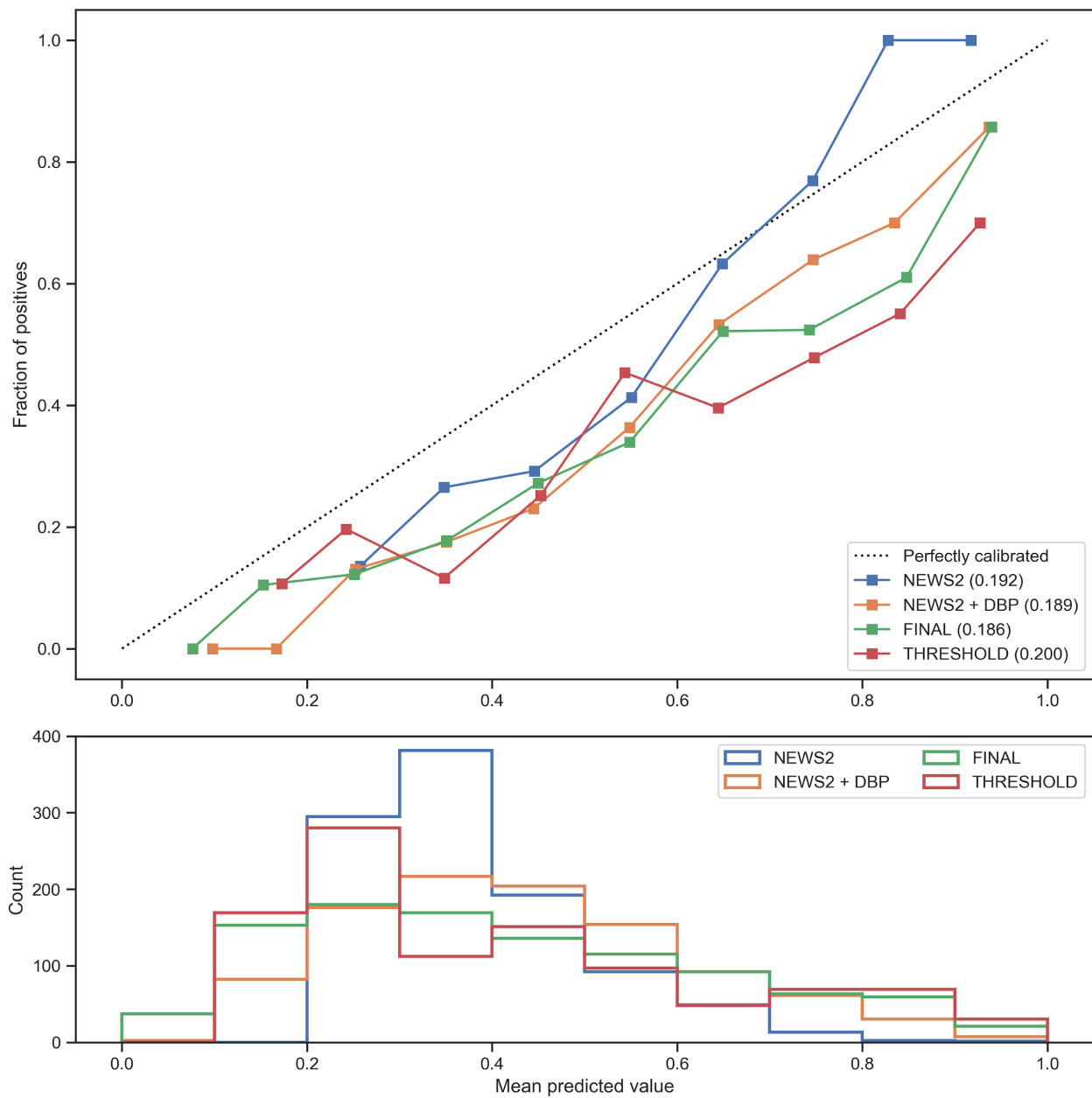
Supplementary Figure 2: Calibration plot from temporal external validation (KCH; n=1025)
