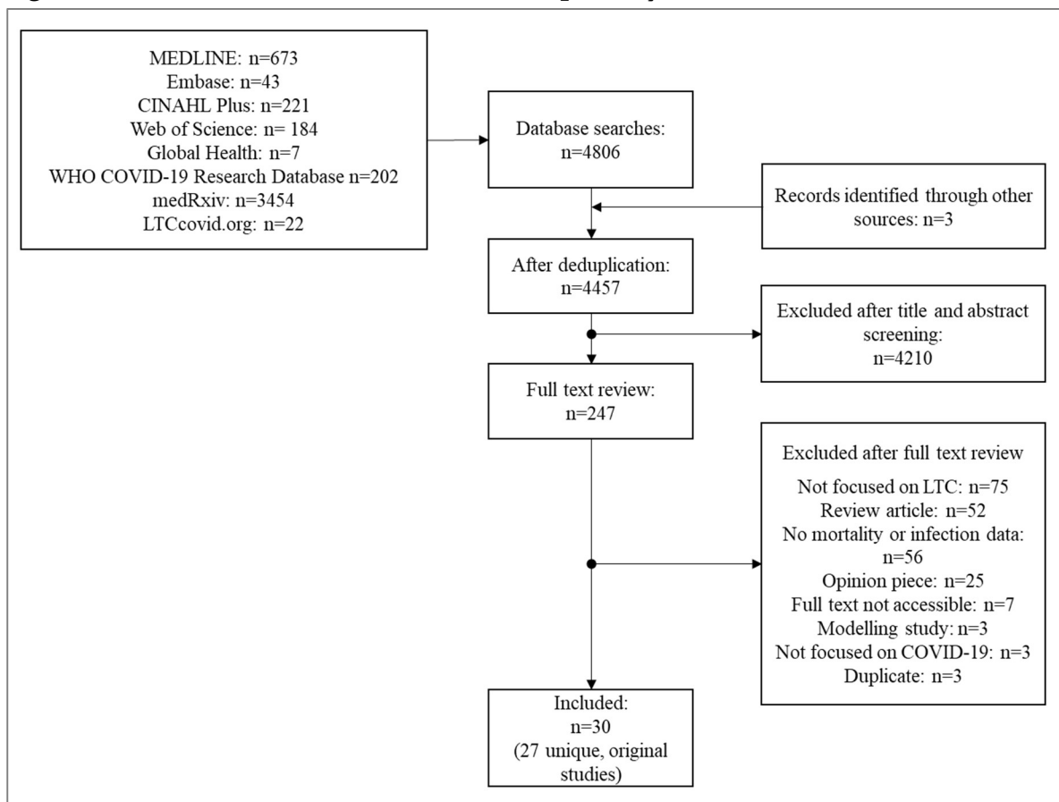
Figure 1: Flow chart for selection of included primary studies
