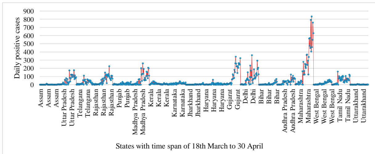
Fig. 4 State wise daily COVID-19 positive cases from 18 th March to 30 th April, 2020
