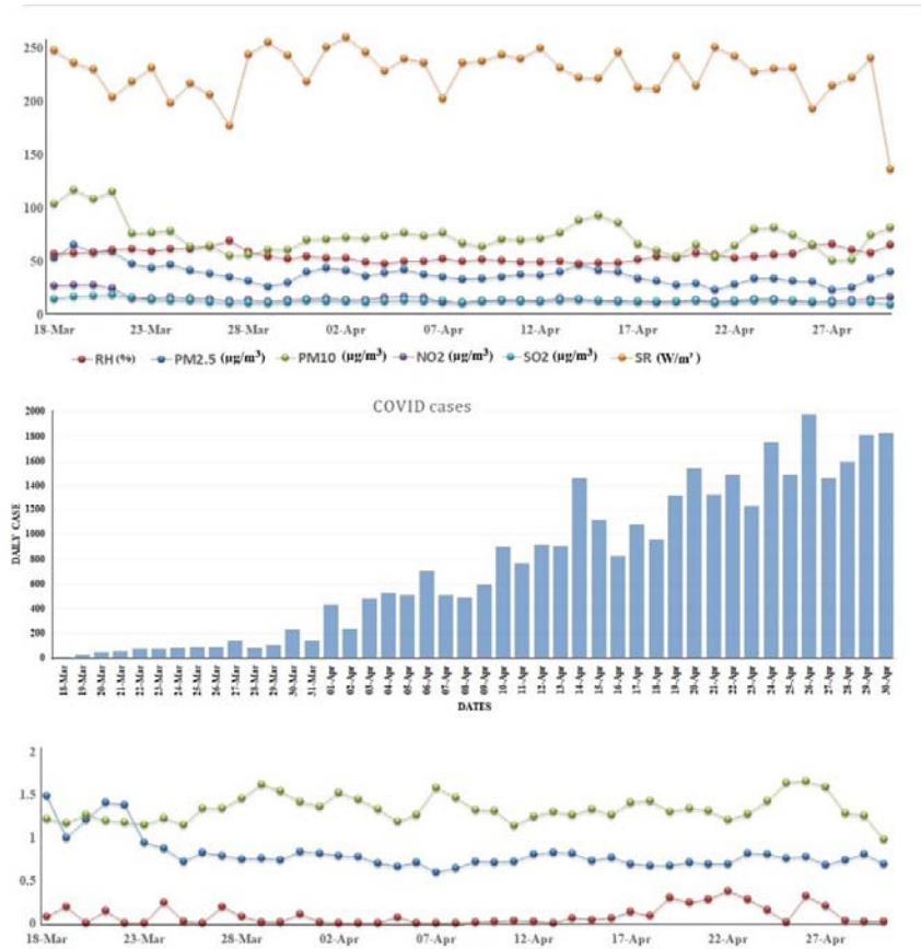
Fig. 3 Temporal distribution of daily COVID-19 cases and mean value of weather parameters and pollutants
