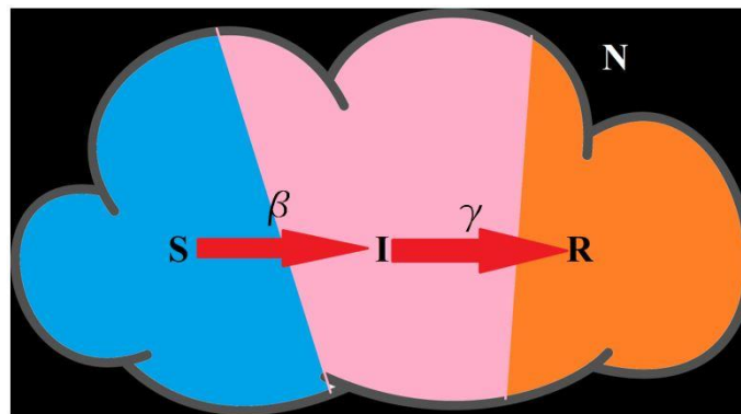
Figure 3: Division of population based on SIR model
