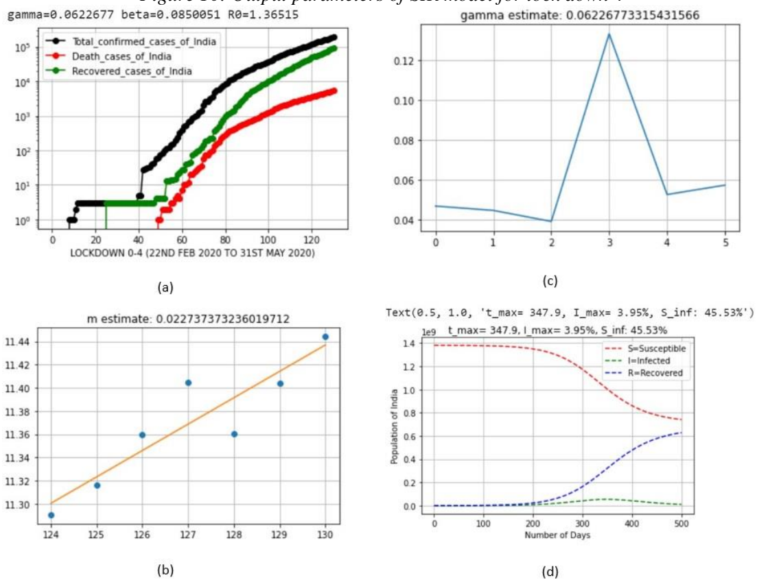
Figure 11: Output parameters of SIR model for lock down 0-4
