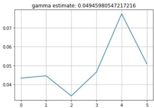
Figure 8: Output parameters of SIR model for lock down 2
