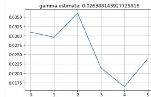
Figure 6: Output parameters of SIR model for lock down 0
