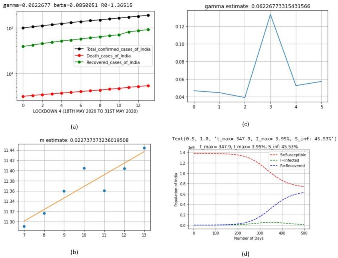
Figure 10: Output parameters of SIR model for lock down 4
