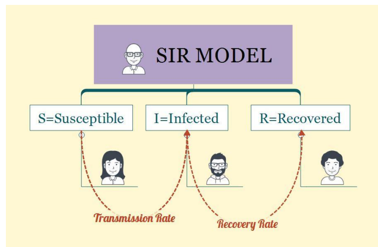
Figure 4: Basic structure of SIR model
