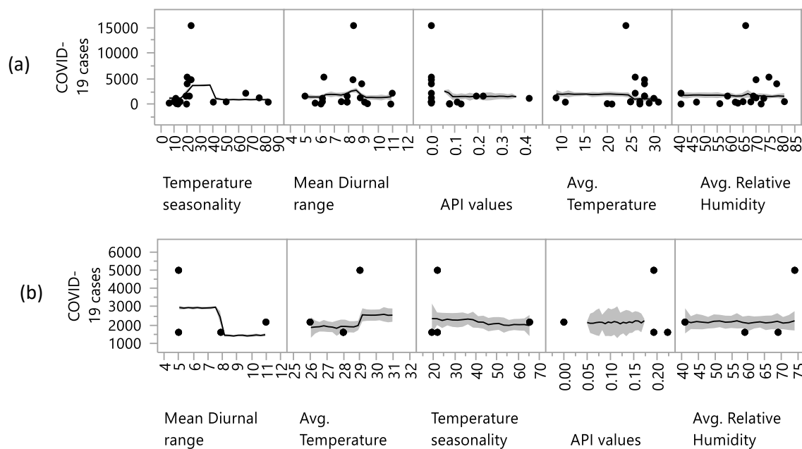
Fig. 7: Marginal dependence graphs for the five most influential predictors in the model for COVID-19 in India (a), Brazil (b). For explanation of predictors and their units, see Table 3. Y-axes are showing COVID-19 cases, and X-axes represent predictors. The predictor, the number of international travelers, was omitted, as it is a primary source of infection, but has no role in community transmission. The value of API was considered in the analysis as these countries are malaria-prone. Shaded line shows a 95% confidence interval from the mean.
