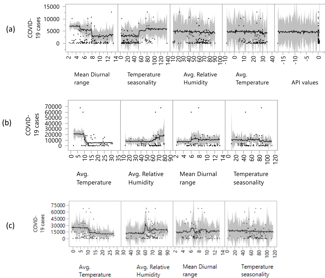
Fig. 5: Marginal dependence graphs for the five most influential predictors in the model for COVID-19 in tropical (a), sub-tropical (b), and temperate (c) regions. For explanation of predictors and their units, see Table 3. Y-axes are showing number COVID-19 cases, and X-axes represent predictors. The predictor, the number of international travelers, was omitted as this is a primary source of infection, but it has no role in community transmission. The API values considered only for the tropical region, where most of the countries of this region are malaria-prone. The shaded line shows a 95% confidence interval from the mean.
