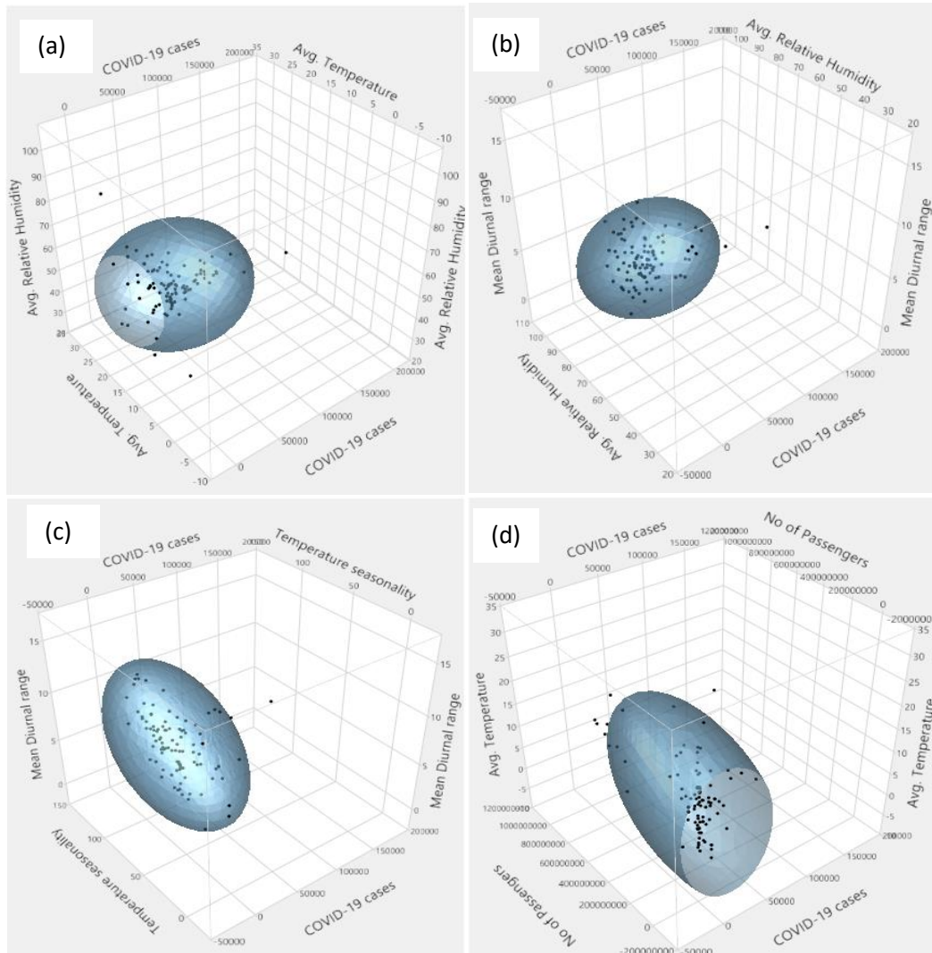
Fig 4: Relationship between selected climatic variables, the number of international travelers, and the number of COVID-19 cases in the temperate region, and a similar relationship has been observed for the sub-tropical region. Fig (a) CoVID-19, relative humidity, and temperature; (b) COVID-19, diurnal range of temperature, and relative humidity; (c) COVID-19, temperature seasonality, and diurnal temperature change; (d) COVID-19, average temperature and API values.
