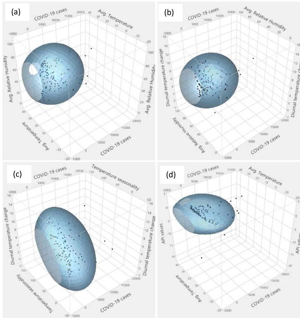
Fig 3: Relationship between selected climatic variables, number of international travelers and number of COVID-19 cases in the tropical region. Fig (a) COVID-19, relative humidity, and temperature; (b) COVID-19, diurnal range of temperature, and relative humidity; (c) COVID-19, temperature seasonality, and diurnal temperature change; (d) COVID-19, average temperature and API values.
