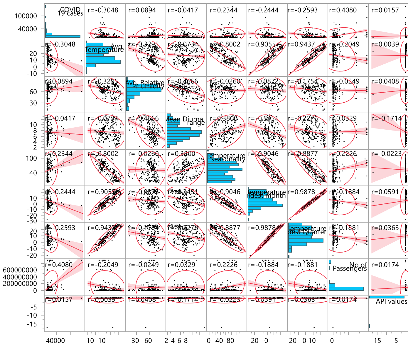
Fig 1: Scatterplot matrix showing the relationship between preliminary predictors and the number of COVID-19 cases. The corresponding correlation value (r) to identify insignificant predictors for the model are shown on the subplots.
