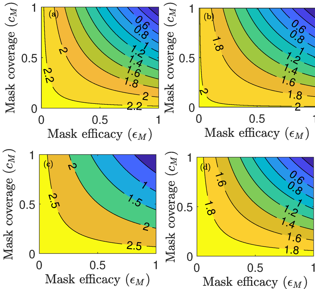
Figure 5: Contour plots of the control reproduction number ( \mathcal{R}_c ) of the model (2.1), as a function of mask coverage ( c_M ) and mask efficacy ( \epsilon_M ), for the special case of the model with no social-distancing. (a) the entire Nigerian nation. (b) Lagos State. (c) Kano State. (d) FCT Abuja. Parameter values used are as given in Tables 4 and 3.
