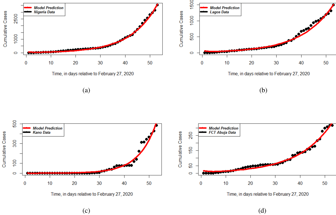
Figure 3: Fitting of the model (2.1) with COVID-19 cumulative data for (a) Nigeria, (b) Lagos State, (c) Kano State, and (d) Federal Capital Territory (FCT) Abuja.
