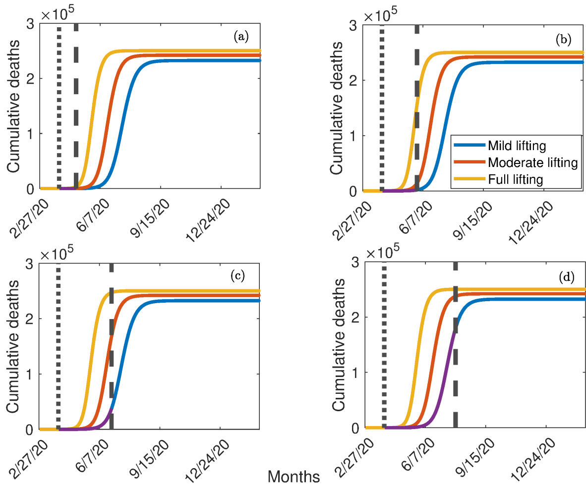
Figure 9: Simulations of the model (2.1), showing cumulative deaths, as a function of time in the absence of mask usage, for the entire Nigerian nation. (a) one month after implementing the lockdown on March 30, 2020 (b) two months after implementing the lockdown on March 30, 2020 (c) three months after implementing the lockdown on March 30, 2020 (d) four months after implementing the lockdown on March 30, 2020. The solid dotted vertical lines indicate the start of the social-distancing lockdown regimen (March 30, 2020), dashed vertical lines indicate when the current strict social-distancing is terminated, and the purple horizontal line segments indicate the duration of the strict social-distancing regimen. Parameter values used are as given in Tables 4 and 3.
