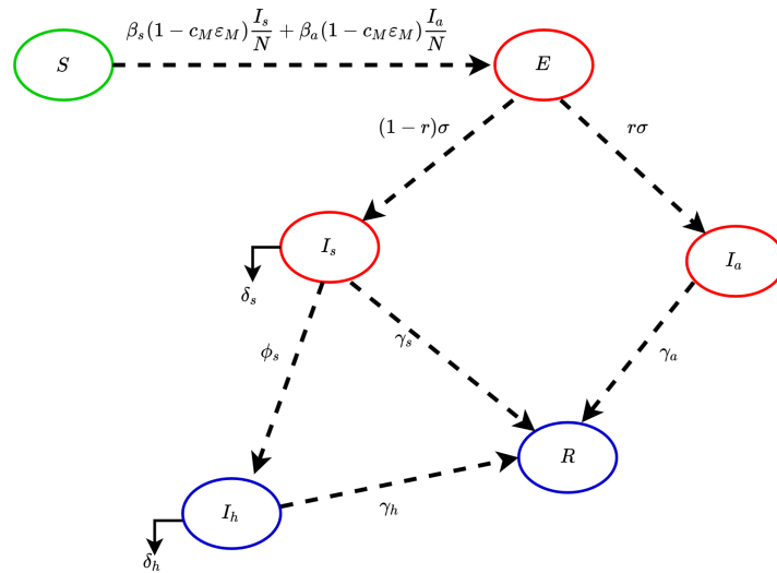
Figure 2: Flow diagram of the COVID-19 model (2.1).
