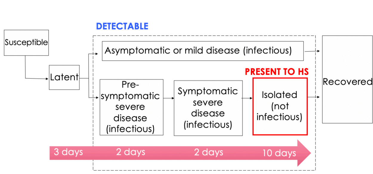
Figure 1. SARS-CoV-2 transmission model schematic. HS: health services.
