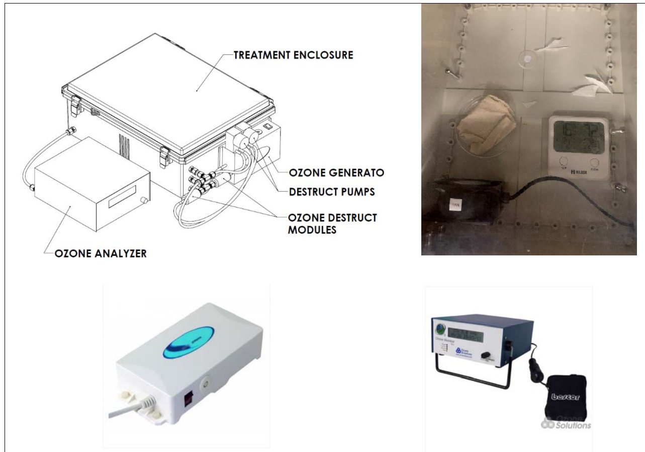
Figure 1 Legend: Ozone Solution's prototype of self-contained ozone chamber. Sealable chamber dimensions: 9" high x 30" deep x 20" wide. Top left: prototype ozone chamber inside fume hood for kill efficacy testing. External ozone analyzer connects to sealed chamber. Top right: inside of sealed chamber, fan at bottom left for ozone circulation, glassware and paper for wicking water to maintain high ambient humidity, hygrometer/thermometer to measure ambient conditions within the chamber during testing. Bottom left: HP-200 (110V/60Hz) low cost ozone generator with air pump. Right: UV-106L ozone concentration analyzer.
