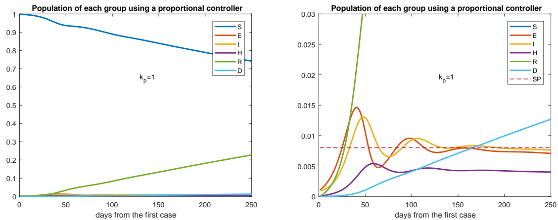
Figure 7: Evolution of every group over time with a proportional control action with gain k_p = 1 (left). The picture at the right is a zoom of that at the left. Set point equal to 0.008.
