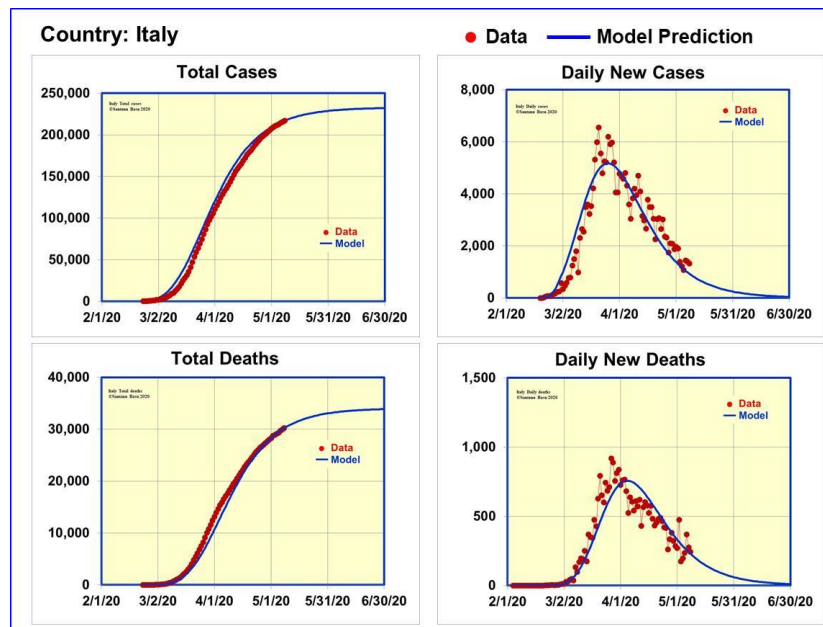
Figure 5. Data and model predictions for Covid-19 cases in Italy
