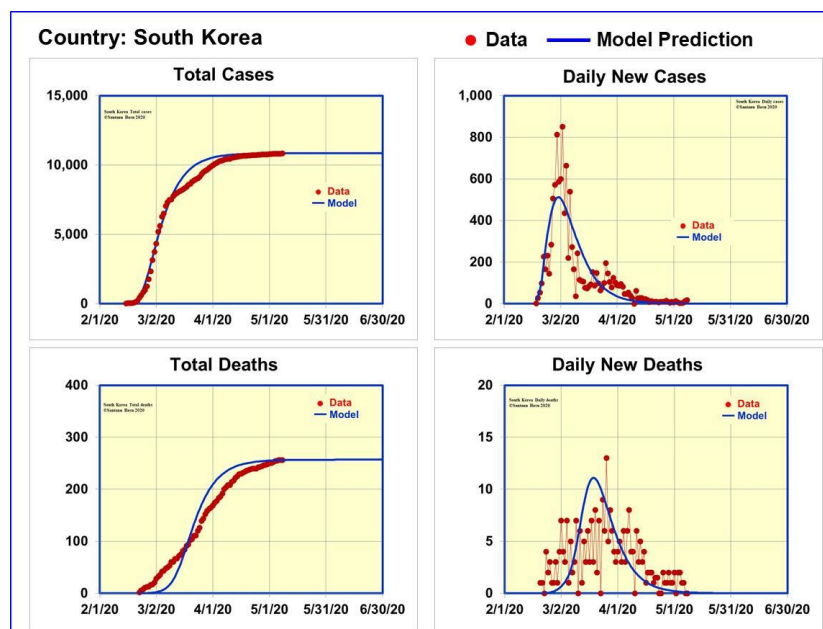
Figure 6. Data and model predictions for Covid-19 cases in South Korea
