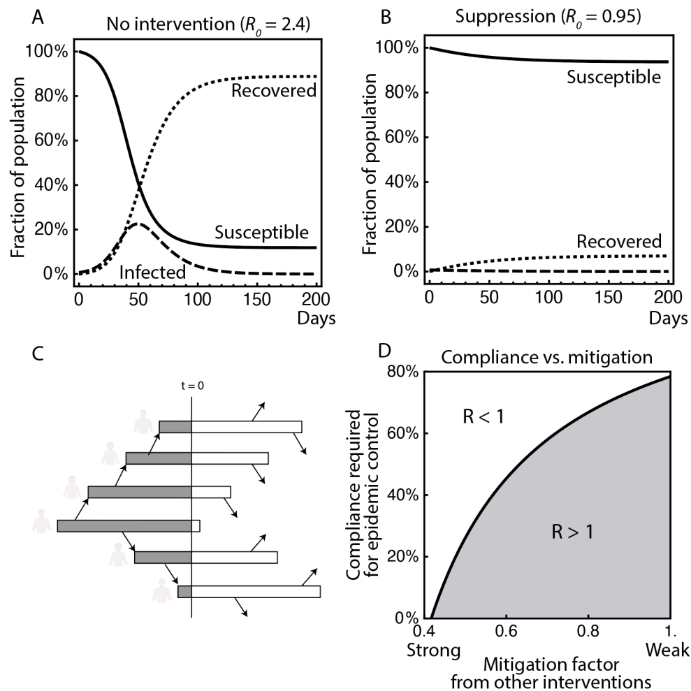
Fig. 1 | Requirements for epidemic control of COVID-19 using population-scale testing and self-isolation. (A) An SIR model 22 with R_0 = 2.4 leads to infection of the majority of the population, with a massive peak of active infection that overwhelms the health care system. (B) With strong interventions that reduce R_0 to 0.95, many deaths are avoided. (C) Testing everyone simultaneously cuts all chains of transmission. (D) The required level of compliance (fraction of all individuals) for effective control of the epidemic, as a function of the strength of other interventions and assuming a test with 85% efficacy (fraction of future infections detected). With moderate social distancing, epidemic control can be achieved even with low levels of test compliance.
