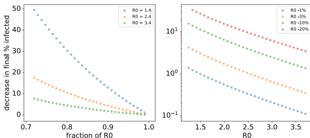
Fig 5 | Consequence of failure to suppress the epidemic by population-scale testing. Left: Decrease in the final attack rate (y-axis) as a function of change in R_0 induced by population-scale testing (x-axis). Note that the effect is nearly linear, and that effects of up to 50% of the total population can be observed even when R_0 remains over 1. Right: Decrease in the final attack rate (y-axis) as a function of initial R_0 that is decreased by 1 to 20% by population-scale testing. The final attack-rates ( z ) were calculated using the lambert W function: z = 1 + W(-R_0 \exp(-R_0)) / R_0 .
