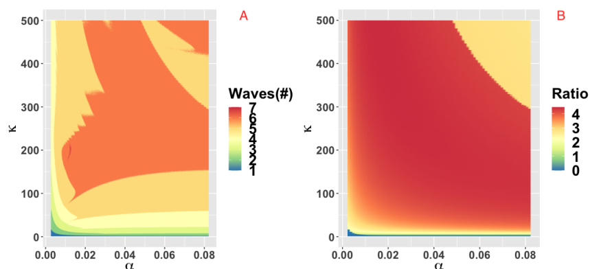
Figure 3: Parameter plane showing model dynamics as they vary with changes in the rate \alpha at which socio-economic losses accrue and the rate \kappa that controls the social learning rate, for the number of COVID-19 waves (a) and the ratio of peak height of the second wave to the first wave peak. Other parameters are at baseline values (Table 1).
