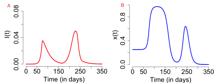
Figure 1: (left) Time series plot of the number of infected individuals in the face of social showing appearance of second wave (left) due to effects of social dynamics (right). The results are obtained for C_0 = 0.6 , R_0 = 2.4 , 1/\sigma = 2.5 , \gamma = 1/5 , \kappa = 5 , \epsilon = 0.008 , \alpha = 1.0 * 24/365 and \delta = 0.05 * 24.0/365 and initial conditions S(0) = (1000000 - 1)/1000000 , E(0) = 0 , I(0) = 1/1000000 , R(0) = 0 , x(0) = 0.25 , L(0) = 0 and H(0) = 0 .
