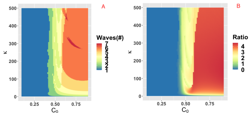
Figure 5: Parameter plane showing model dynamics as they vary with changes in the rate \kappa that controls the social learning rate and the parameter C_0 which controls how effective closure is, for the number of COVID-19 waves (a) and the ratio of peak height of the second wave to the first wave peak. Other parameters are at baseline values (Table 1).
