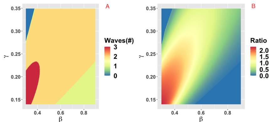
Figure 2: Parameter plane showing model dynamics as they vary with changes in the transmission rate \beta and the rate \gamma at which the infectious period ends, for the number of COVID-19 waves (a) and the ratio of peak height of the second wave to the first wave peak. Other parameters are at baseline values (Table 1).
