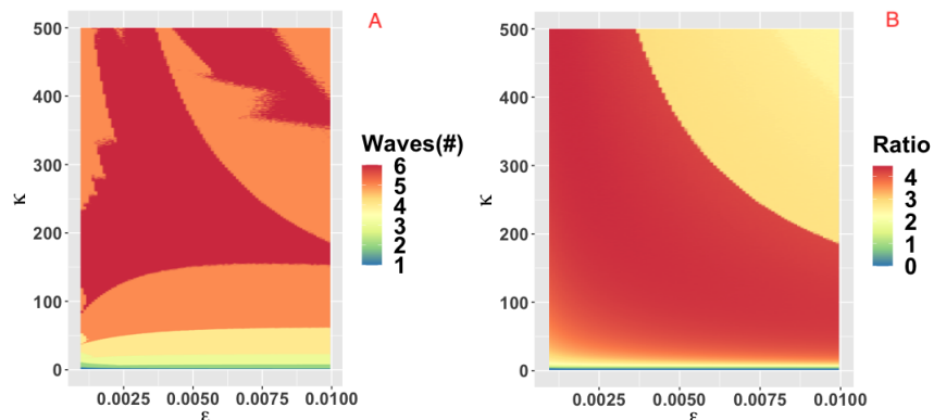
Figure 4: Parameter plane showing model dynamics as they vary with changes in the rate \kappa that controls the social learning rate and the parameter \epsilon which controls how sensitive the population is to economic losses relative to infection prevalence, for the number of COVID-19 waves (a) and the ratio of peak height of the second wave to the first wave peak. Other parameters are at baseline values (Table 1).
