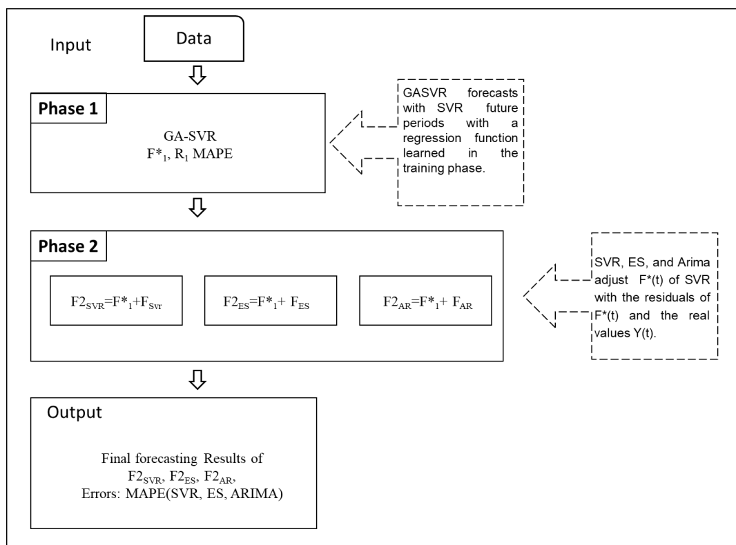
Figure 1. SVR-ESAR Architecture.
