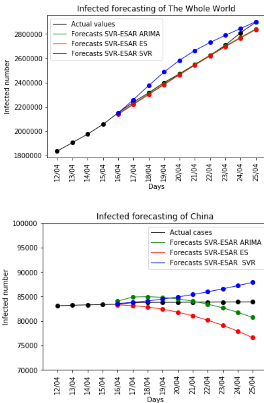
Figure 2: Forecast of SVR-ESAR for the Whole World and China
