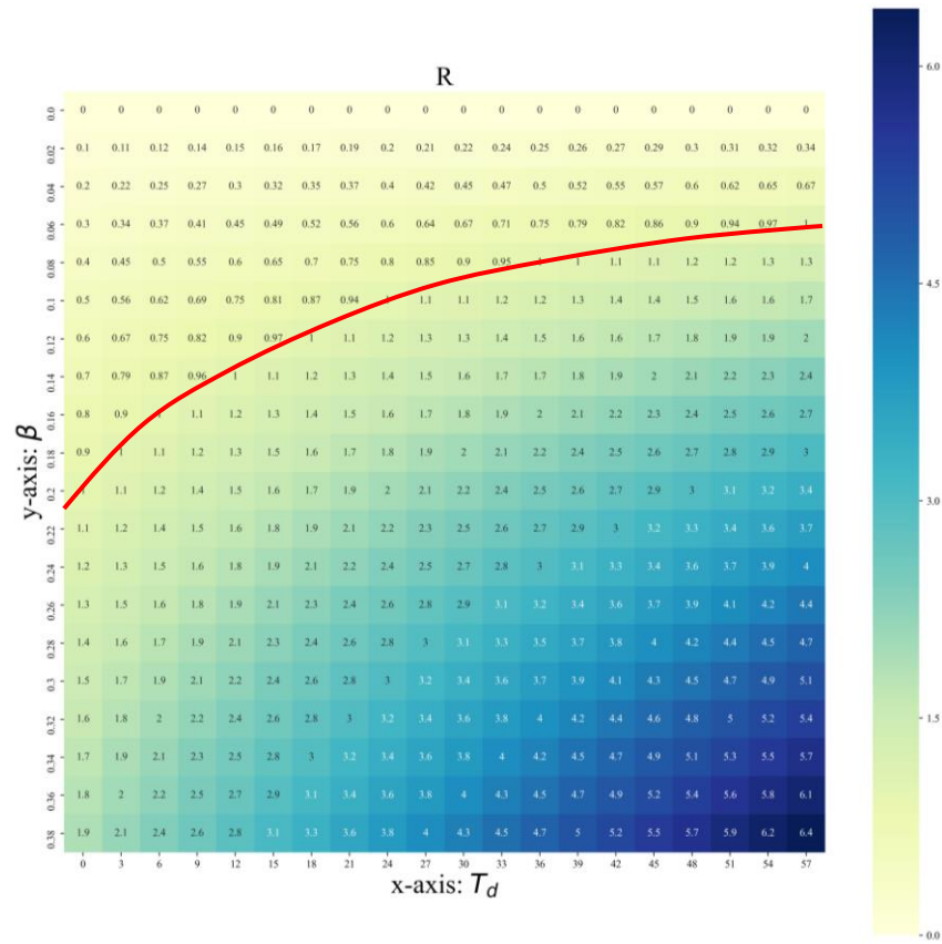
Figure 14. Sensitivity analysis of estimated R value with different \beta and T_d . R at the red line position is equal to 1.
