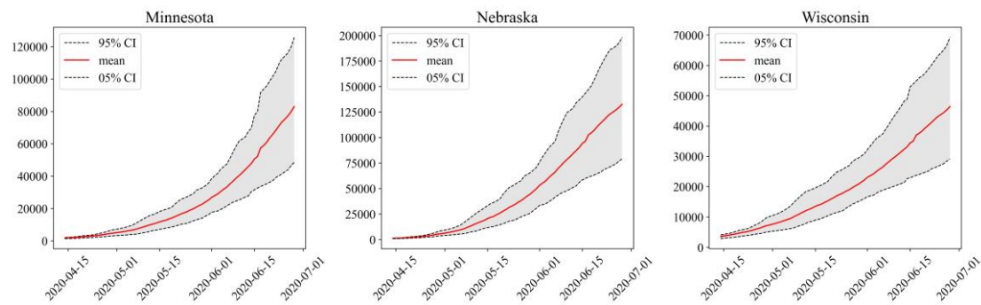
Figure 10. Based on the data from March 21 to April 13, 2020, the cumulative number of confirmed cases in three potentially risky states: Minnesota, Nebraska and Wisconsin, was predicted. The x-axis represents time. The y-axis represents number of people.
