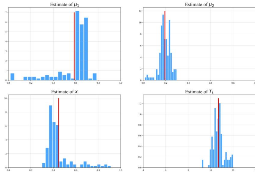
Figure 8. Frequency histogram of the estimated \mu_1 , \mu_2 , x , T_L after t_0 . The x-axis means the value and y-axis means the frequency density. The red vertical line represents the mean value.
