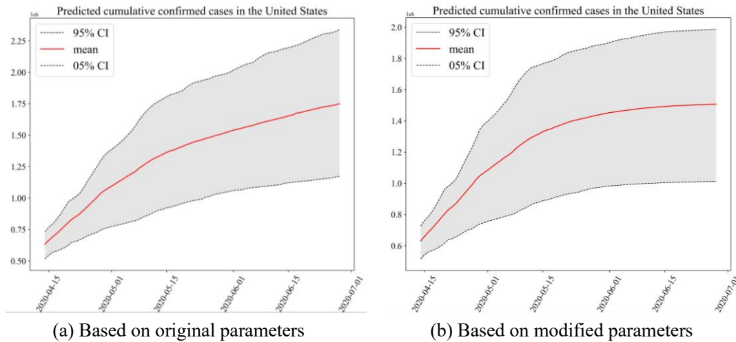
Figure 12. Based on the data from March 21 to April 13, 2020, the cumulative number of confirmed cases in the United States was predicted. The x-axis represents time. The y-axis represents the number of people. (a) The simulation is based on the parameters estimated by the original model. (b) The simulation is based on the estimation parameters of the model after forced suppression process. The estimated parameter c of Minnesota, Nebraska and Wisconsin was doubled, and \beta was reduced by 0.2.
