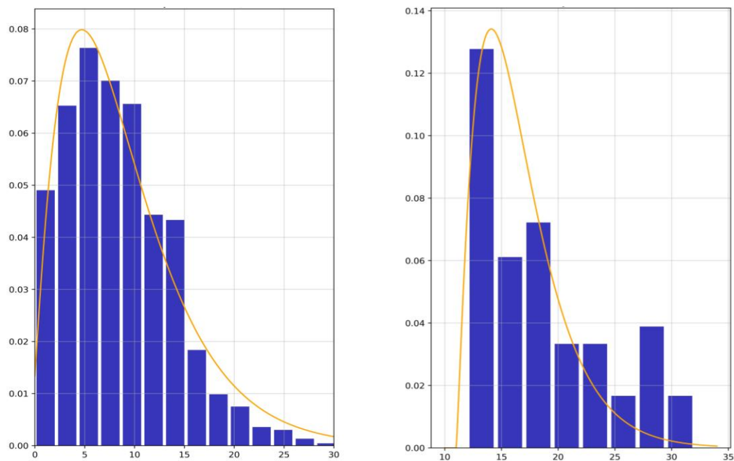
Figure 2. Left subgraph is the sample and probability distribution of T_d , and right subgraph is the sample and probability distribution of T_l . The orange curve represents the estimated probability distribution, and the blue column represents the statistical samples.
