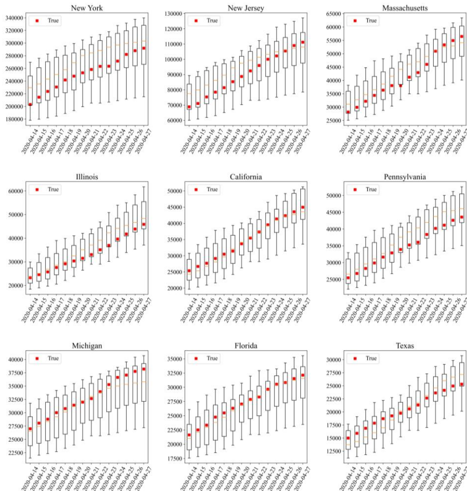
Figure 9. True data from several major states in the United States are compared with estimated results in the two weeks after April 13. The red blocks represent the observed true cumulative confirmed data, and the box charts represent the results of 10 independent predictions.
