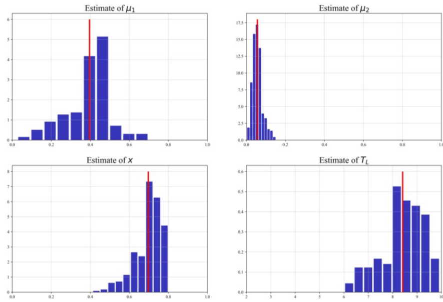
Figure 6. Frequency histogram of the estimated \mu_1 , \mu_2 , x , T_L before t_0 . The x-axis means the value and y-axis means the frequency density. The red vertical line represents the mean value.
