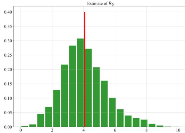
Figure 4. Frequency histogram of the estimated R_0 . The x-axis means the value of R_0 and y_axis means the frequency density. The red vertical line represents the mean value of R_0 .
