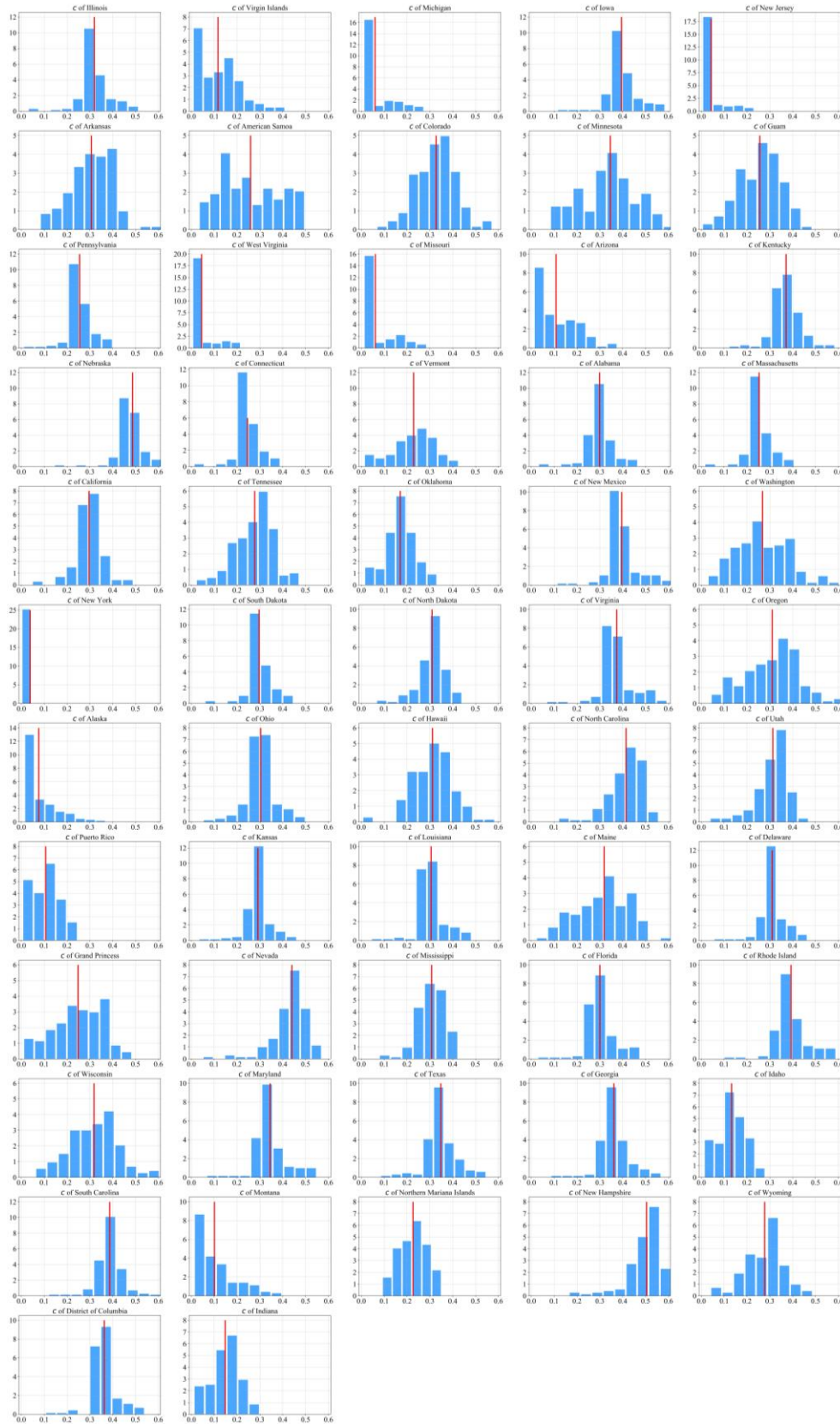
Figure 7. Frequency histogram of the estimated c in 57 states in the United States after t_0 . The x-axis means the value of c and y-axis means the frequency density. The red vertical line represents the mean value of c .
