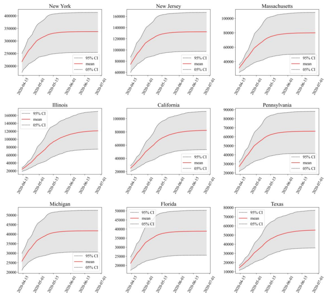
Figure 11. Based on the data from March 21 to April 13, 2020, the cumulative number of confirmed cases in 9 states with most severe outbreaks of COVID-19 was predicted. The x-axis represents time. The y-axis represents the number of people.
