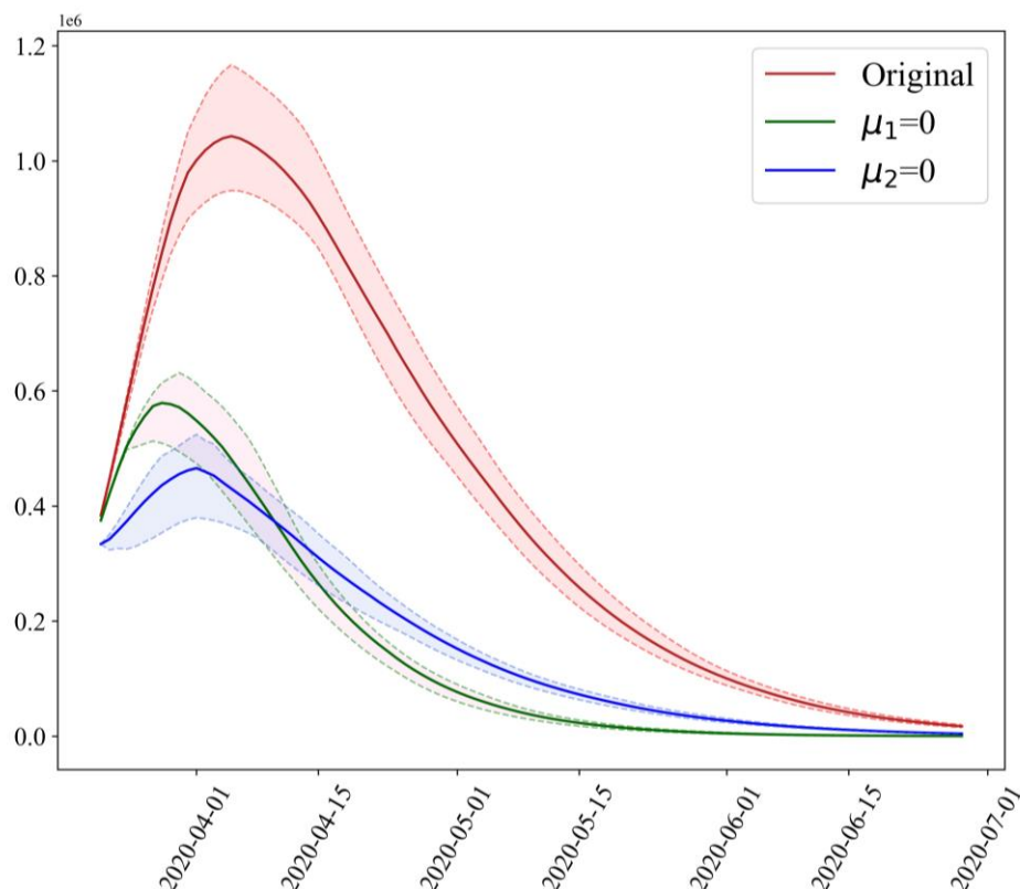
Figure 13. Estimates of the number of patients with incubation period over time in the United States. The x-axis represents time and the y-axis represents the number of people. The solid lines of the same color system represent the mean value, and the dotted lines represent 95% CI and 5% CI.
