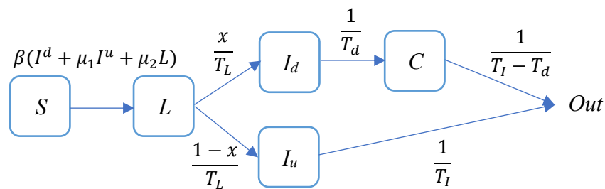
Figure 1. State transition diagram of transmission dynamics system.
