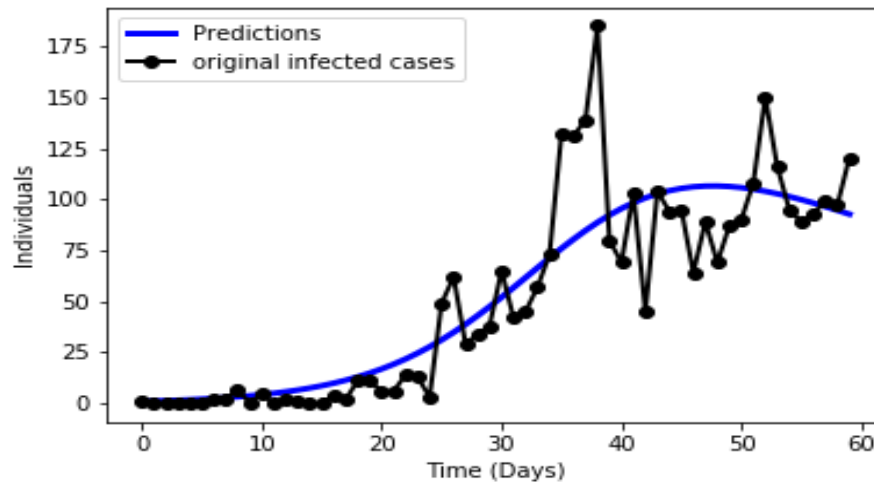
Figure 1: Fit of the optimal SIR model for Algeria infected cases with covid-19, from 25 February 2020 to 24 April 2020
