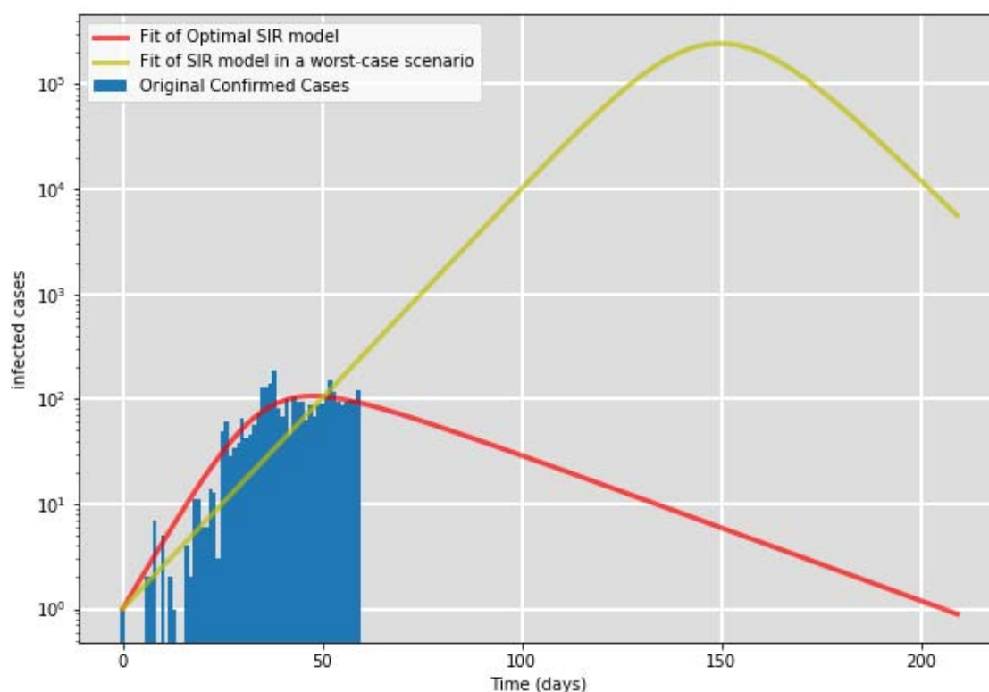
Figure 3: Prediction of the epidemic peak of COVID-19 in Algeria by fitting an optimal SIR model and an SIR model in a worst-case scenario.
