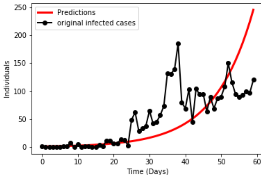
Figure 2: Fit of SIR model for Algeria infected cases in a worst-case scenario covid-19, from 25 February 2020 to 24 April 2020.
