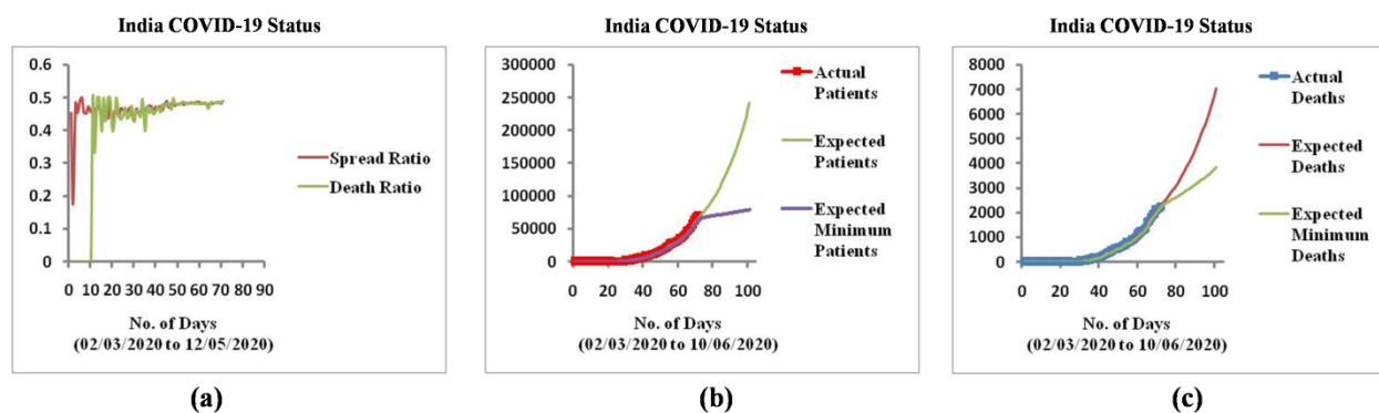
Figure 1(a) Spread and death ratio of COVID-19 in India. (b) Prediction curves for expected patients of COVID-19 in India. (c) Prediction curves for deaths of COVID-19 in India.
