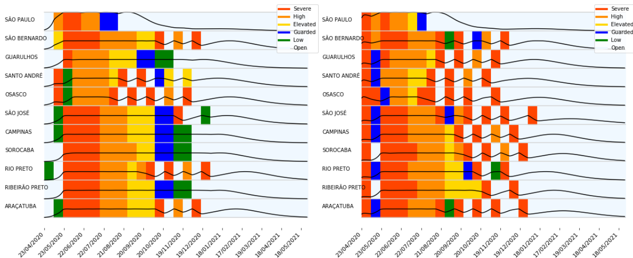
Figure 4: Prediction of optimal control for major cities in the state of São Paulo. The protocol changes every two weeks and optimizes the level control and the timing to apply the control measures. Thus each city can meet its own needs to curb the spreading. In the left inset, we show the optimal control taking into account the official data. In the right inset, we take into account a sub-notification.
