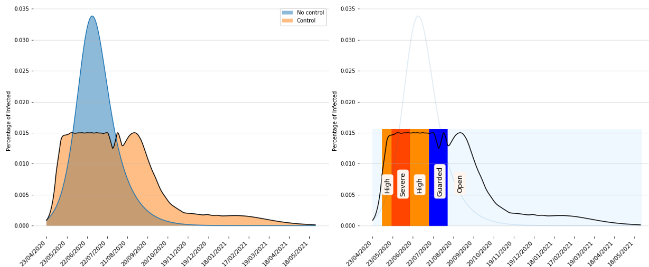
Figure 3: Impact of the optimal control protocol implemented in the State of São Paulo. The control protocol does not allow for the infected population in the city of São Paulo to surpass 1.5% and in the countryside 0.7% (this would roughly correspond to take campaign hospitals into consideration). In the left inset, we show the situation with social distancing only (blue) and with optimal control (beige) where the infected population never exceeds 1.5% as set in the control. In the right inset, our approach provides levels of control for the city of São Paulo. This prediction performed using the official government data.
