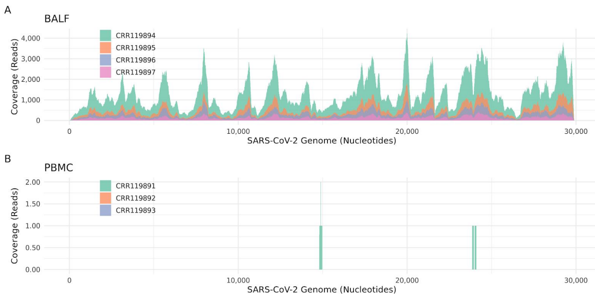
Figure 2. Mapping of SARS-CoV-2 RNA against the SARS-CoV-2 genome
