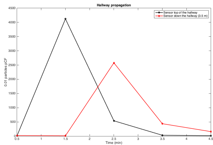
Figure 5. Source in closed-hallway and its propagation down the hallway at marker 6 and 12 locations in Figure 3 : convection of the signal down the hallway and an exponential dampening of the signal was observed.
