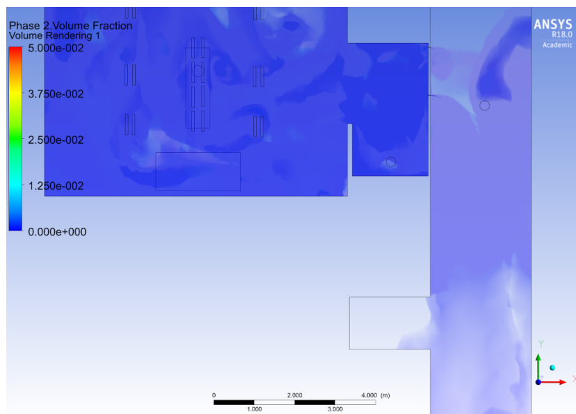
Figure 2. CFD simulation tracking the CO 2 source emitted at the OR table; in the CFD simulation, injection is done for 10 seconds at the beginning of the simulation. The door of the OR is closed, while the door of the adjacent OR is open. This figure shows that the plume reaches the adjacent OR after 130 sec.
