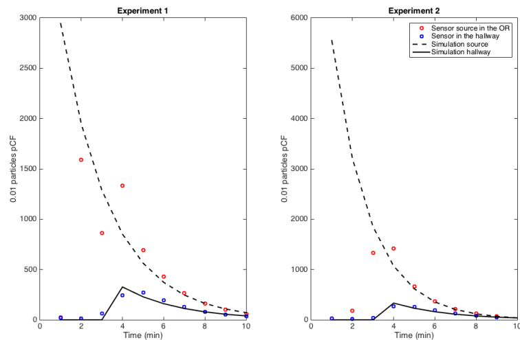
Figure 4. Source in closed-door OR and its impact on hallway air concentration: a 2 min delay in transmission from OR to hallway and an exponential decay for each signal was observed.
