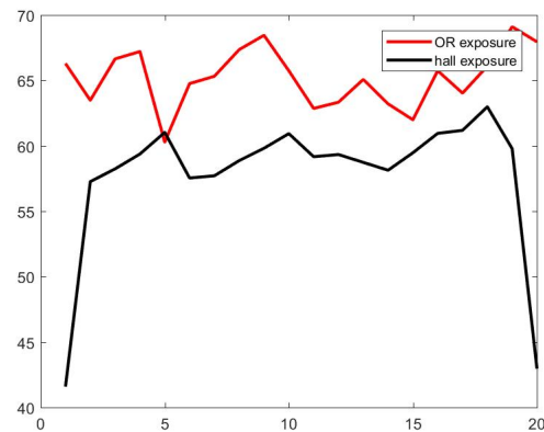
Figure 10. Effect of the frequency of door openings on the concentration of pollutants (y-axis) in each OR (x-axis) and in the respective portion of hallway. Here the frequency is set at 2 min .
