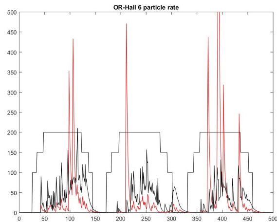
Figure 8. Result of the simulation of three surgeries using the model with stochastic production of smoke and opening of door linked to the status of the surgery. The steps follow: Patient in (100) - Patient extubated (150) - Start laparoscopic portion (200) - Stop laparoscopic portio - Patient extubated - Patient out.
