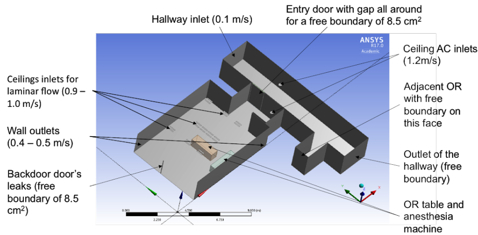
Figure 1. 3-Dimensional model of the OR and adjacent hallway.
