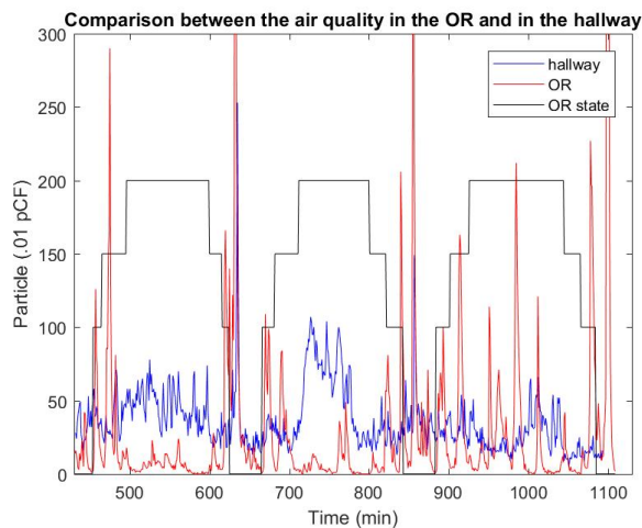
Figure 7. Measurement of the air quality in the OR and in the hallway compared with the status of the surgery. Here, three laparoscopic surgeries are analysed. The steps follow: Patient in (100) - Patient extubated (150) - Start laparoscopic portion (200) - Stop laparoscopic portio - Patient extubated - Patient out.
