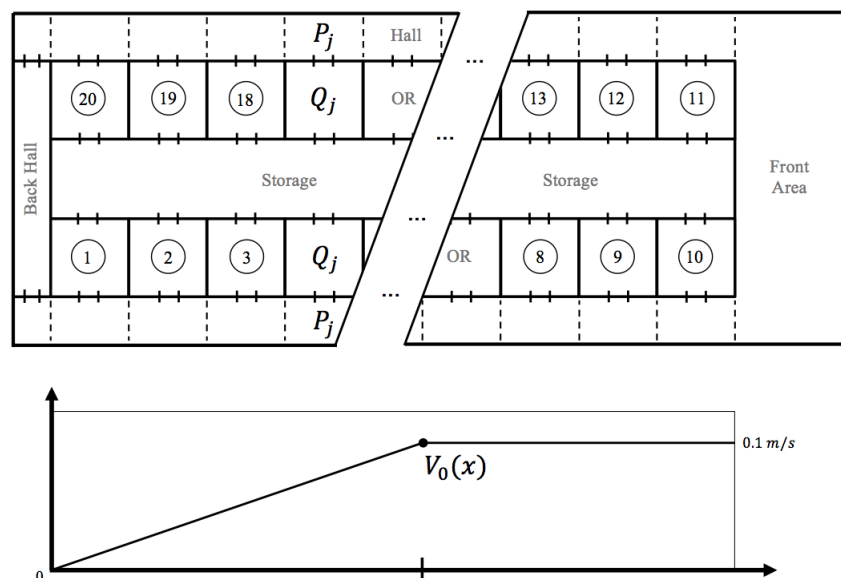
Figure 13. Approximate floor plan of the surgical suite used during the clinical test. The dash lines represent the coarse finite volume grid used for the diffusion transport equation in the hallway. v_0(x) is the velocity of the airflow moving down the hallway.
