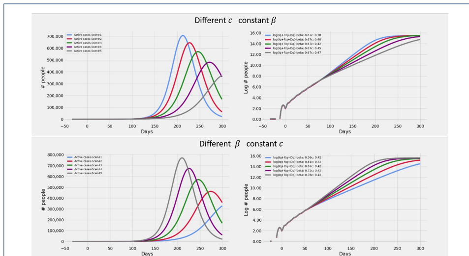
Figure 4 Effect of varying \beta with a constant intervention: Plots showing (a) Evolution of active cases of infected persons at various c and constant \beta (b) Cumulative number of cases over a 300 day epoch on log scale at various c and constant \beta (c) Evolution of active cases of infected persons at various \beta and constant c (d) Cumulative number of cases over a 300 day epoch on log scale at various \beta and constant c . All simulations start with the same values of \beta and c . The variations of \beta and c are applied on day 50 (See Methods for values of parameters used)
