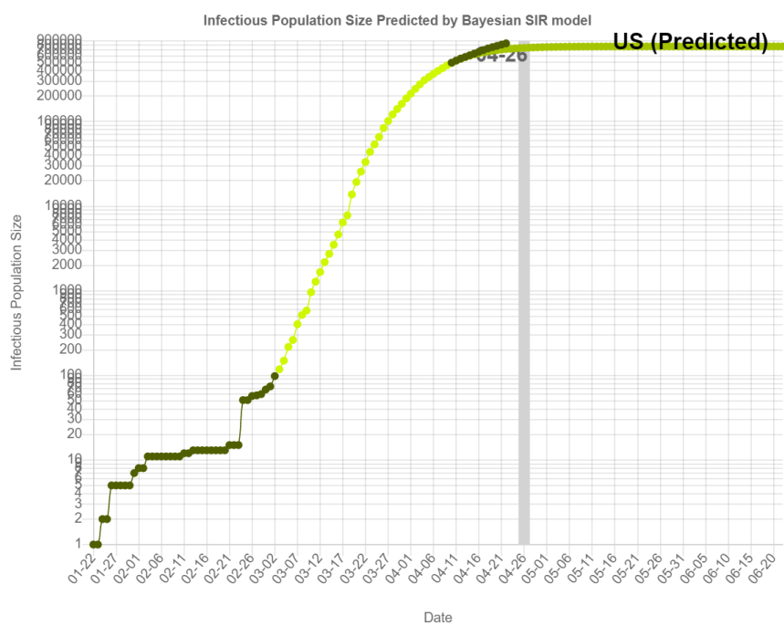
Figure 6: Prediction of the cumulative number of individuals in United States, estimated using the data up to April 23rd.
