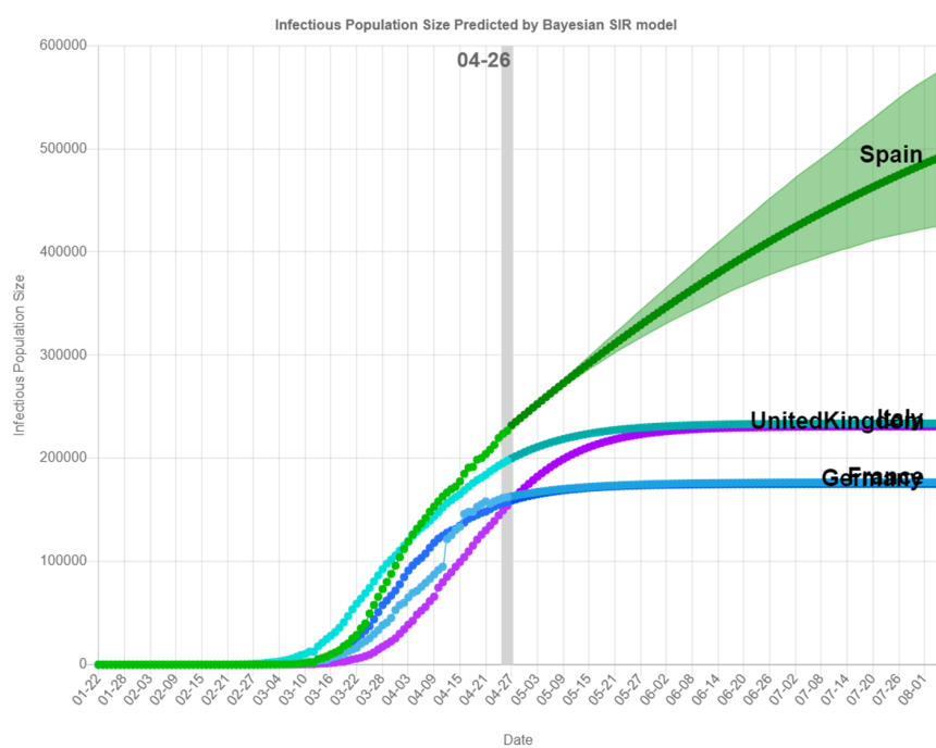
Figure 8: Prediction of the cumulative number of individuals in European countries, estimated with the data up to April 26th.
