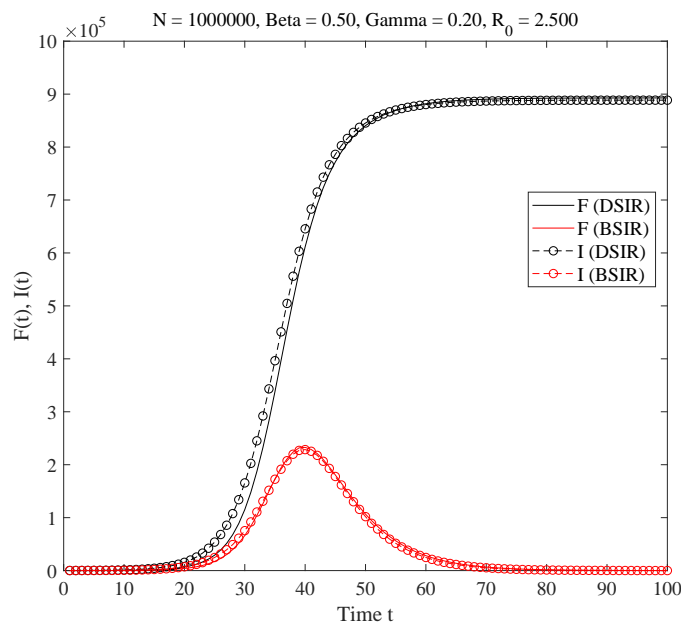
Figure 1: The cumulative number of infected individuals F(t) = N - S(t) and the number of infected individuals I(t) in DSIR and BSIR model.
