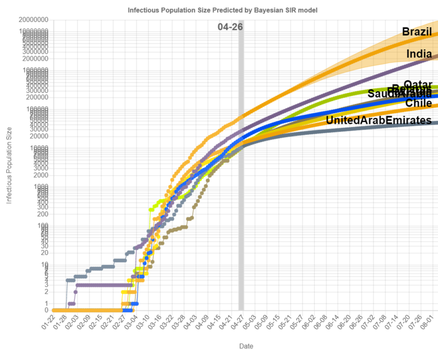
Figure 9: Prediction of the cumulative number of individuals in the countries (Brazil, India, Saudi Arabia, Chile, Pakistan, United Arab Emirates, Belarus, and Qatar, in the descending order at the data analyzed) with predicted increase, estimated with the data up to April 26th.
