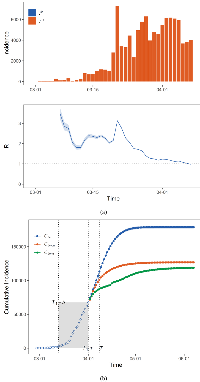
Figure 4: (a) Evolution of the number of cases and the time-varying reproduction number R(t) in Germany. (b) Accumulated case numbers at a time T and at the end of epidemics based on extrapolated R_{de}(t) (blue line), R_{de-cn}(t, \tau) (orange line), and R_{de-kr}(t, \tau) (green line).
