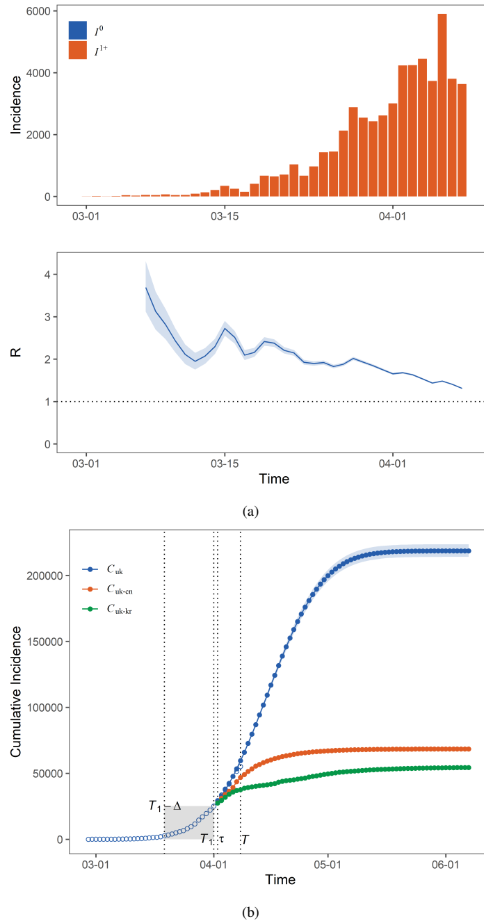
Figure 6: (a) Evolution of the number of cases and the time-varying reproduction number R(t) in UK (b) Accumulated case numbers at a time T and at the end of epidemics based on extrapolated R_{uk}(t) (blue line), R_{uk-cn}(t, \tau) (orange line), and R_{uk-kr}(t, \tau) (green line).
