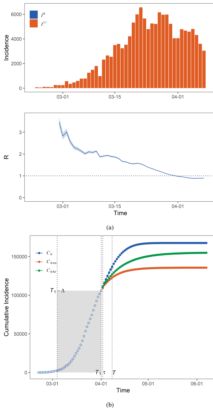
Figure 8: (a) Evolution of the number of cases and the time-varying reproduction number R(t) in Italy (b) Accumulated case numbers at a time T and at the end of epidemics based on extrapolated R_{it}(t) (blue line), R_{it-cn}(t, \tau) (orange line), and R_{it-kr}(t, \tau) (green line).
