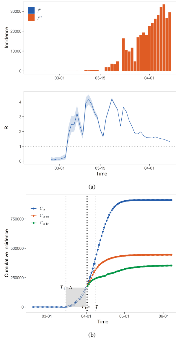
Figure 2: (a) Evolution of the number of cases and the time-varying reproduction number R(t) in the US. Shaded regions of R(t) mark the 95% prediction envelopes. (b) Accumulated case numbers at a time T and at the end of epidemics based on extrapolated R_{us}(t) (blue line), R_{us-cn}(t, \tau) (orange line), and R_{us-kr}(t, \tau) (green line). \tau indicates the time that effective actions were taken. The extrapolated R_{us}(t) makes use of actual data in t \in [T_1 - \Delta, T_1] , where T_1 < T so that we can compare the extrapolated R_{us}(t) and the actual t \in [T_1 - \Delta, T_1] .
