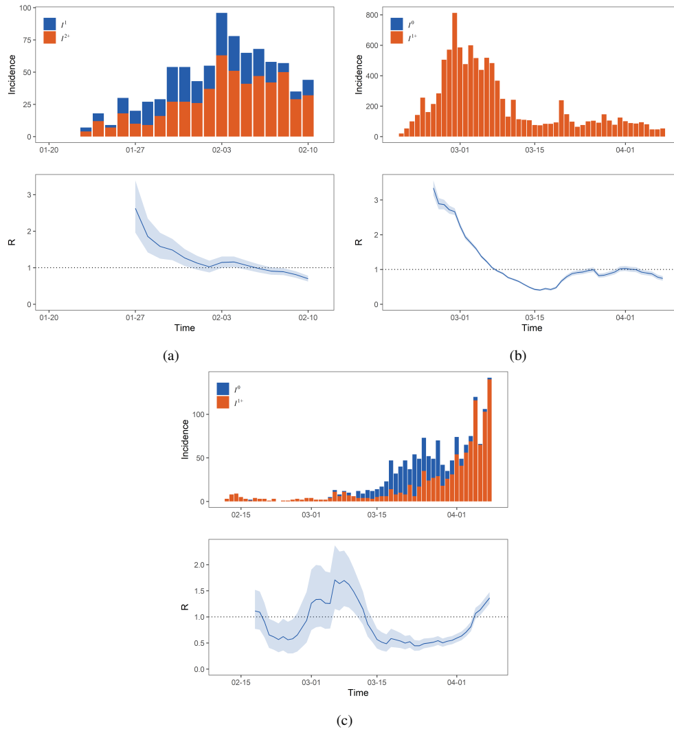
Figure 1: Evolution of the number of cases and the time-varying reproduction number R(t) in China (a), South Korea (b), and Singapore (c). I^0(t) , I^1(t) and I^2(t) denotes respectively the imported thus the zeroth-generation cases, the local cases infected by the imported cases thus the first-generation cases, and the cases infected by the first-generation cases, and the cases infected by the first-generation cases thus the second-generation cases. A notation I^{n+}(t) refers to the n -th and higher generations. Shaded regions of R(t) mark the 95% prediction envelopes.
