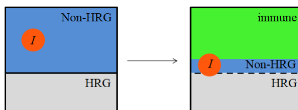
Figure 3: Illustration of the divide and conquer scenario. The whole population is initially split into a high risk group (HRG) and a non-HRG. Infectious individuals are assumed to exist only among the non-HRG, while the HRG is strictly isolated. As time evolves most of the non-HRG become immune. The HRG is released from the isolation if \mathcal{R}_{\text{eff}} < 1 can be ensured due to the large fraction of immune people.
