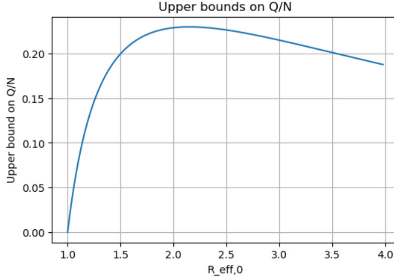
Figure 4: Upper bounds of Q/N as a function of \mathcal{R}_{\text{eff},0} .
