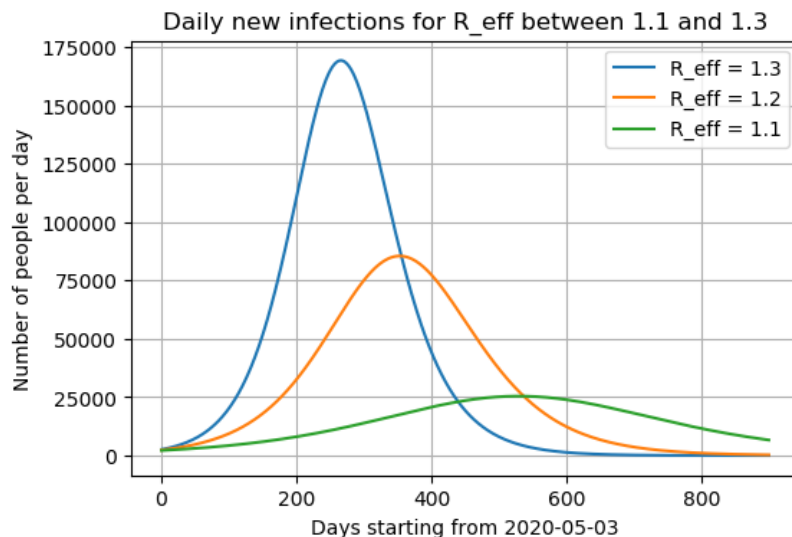
Figure 2: This plot shows the expected daily infections for the Covid-19 pandemic in Germany for \mathcal{R}_{\text{eff}} between 1.1 and 1.3. The initial conditions were set by the publicly available data for 2020-05-03 [35].
