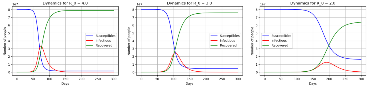
Figure 1: These plots show the dynamics of the Covid-19 pandemic for reproduction numbers \mathcal{R}_0 \in \{2.0; 3.0; 4.0\} . The number of susceptible (blue), infectious (red) and recovered (green) people is plotted against time (in days). It is emphasised that these plots are not suitable for predictions. Instead they merely reveal the underlying dynamics of the SIR-model.
