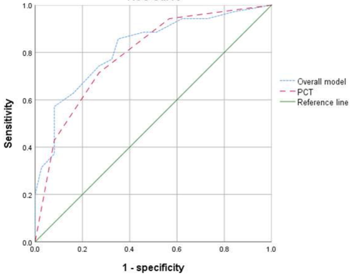
ROC Curve
