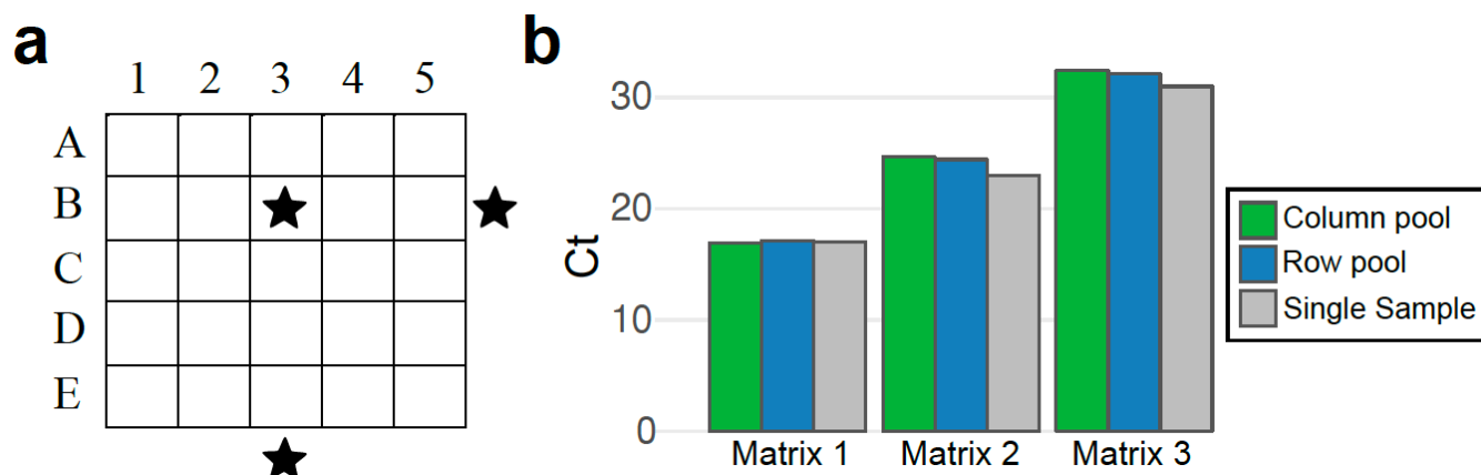
Figure 2: Matrix pooling. (a) Scheme for 5x5 matrix pooling. 25 samples sorted in a 5 x 5 matrix and each row and each column is pooled into a total of 10 pools, on which RNA extraction, reverse transcription and qPCR are performed. In this illustration row B and column 3 are positive (black stars), hence sample B3 is the only positive sample. If more than one row and one column are positive then all the samples in the intersection need to be retested, as some may be negative. (b) Three 5x5 pool matrices were generated (30 pools from 75 lysates). Each matrix (25 lysates that were previously tested individually) included a single lysate positive for SARS-COV-2. As expected, only 6 pools (one row and one column per matrix) were positive for SARS-COV-2, while 24 pools had Ct >40 (Undetected). RT-PCR Ct values of positive pools were nearly identical in the column pool (green) and the row pool (blue), and similar to the values of the individual test of the positive sample (gray).
