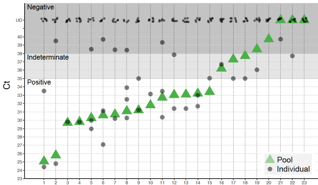
Figure 1: Pooling 8 lysates retain clinical sensitivity. Shown are results of 23 pooling experiments, with 8 lysates in each pool; 15 pools with positive samples indeed come up positive (pools 1-15), 3 pools without positive samples come up negative (pools 20, 21, 23), and 4 out of 5 pools containing a single indeterminate sample detected as indeterminate (pools 16, 17, 18, 19, 22); Pools containing 1-2 samples with low amount of SARS-CoV-2 are detected at a similar Ct (pools 9-18), showing clinical sensitivity is retained and the risk of false negatives is minimal. UD= Undetected.
