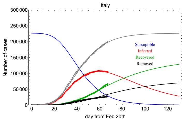
Figure 4: Fit with the SIRD-T model for Italian data since February 20th, 2020.
