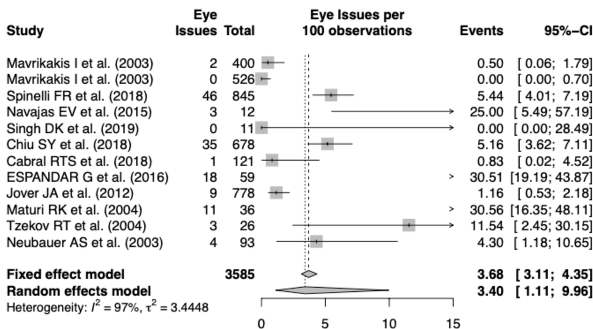
Figure 3: Forest plot for our RMA
