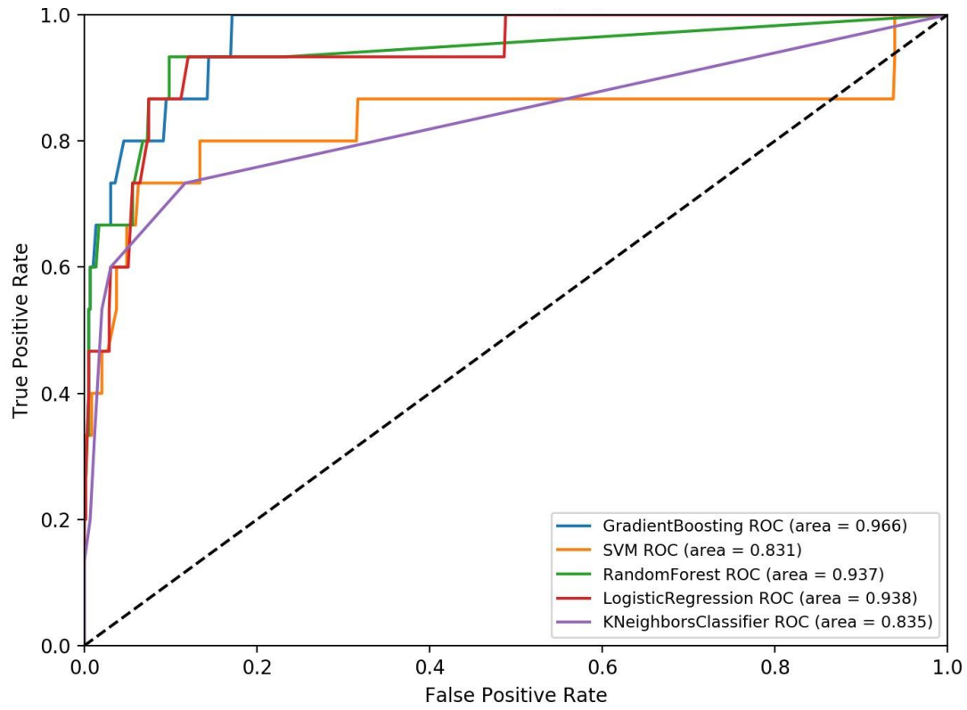
Figure 2. ROC and AUC of machine learning algorithms
