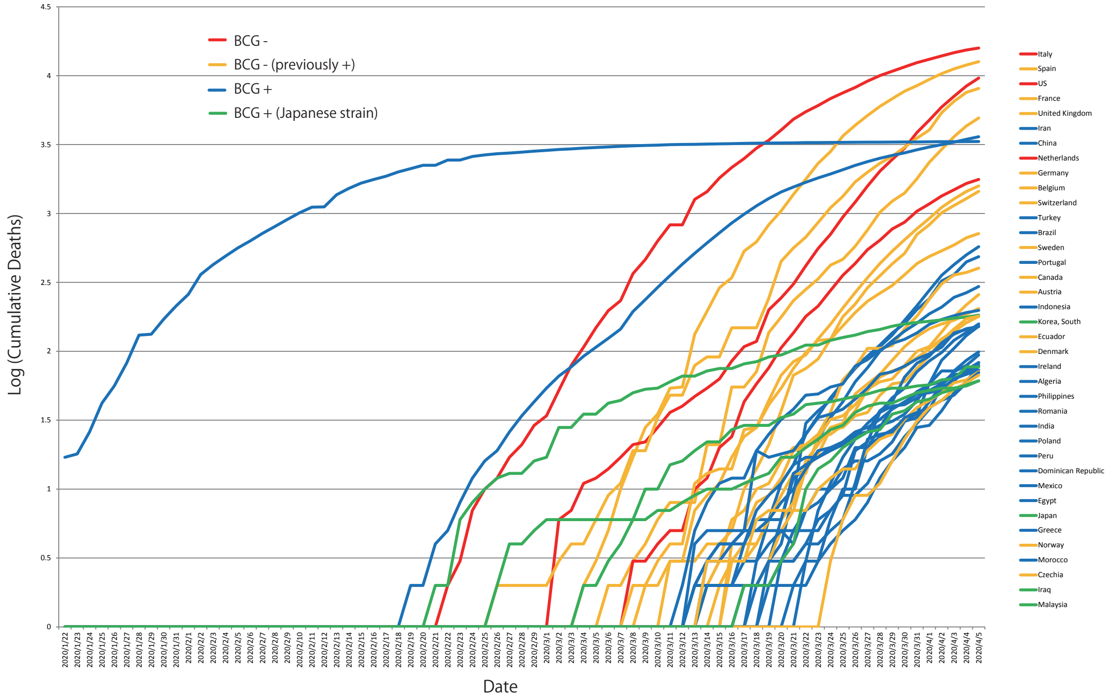
Fig. 7. Cumulative deaths of nations (total deaths over 25). Although the increase rate in Iraq, Korea, and Japan seem to low, at the beginning of the increase, the rate is not particularly low. Malaysia which uses Japanese strain shows a similar pattern to the other nations.
