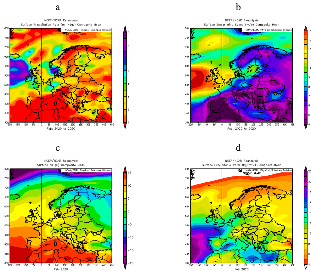
Figure 2. Mean values of several meteorological variables for February 2020 over Europe. a) Precipitation rate (mm/day), b) Surface wind speed (m/s), c) Surface air temperature (°C), and d) Precipitable water ( \text{kg/m}^2 ). Image generated with the Web-based Reanalysis Intercomparison Tool provided by the NOAA/ESRL Physical Sciences Laboratory, Boulder Colorado from their Web site at http://psl.noaa.gov/
