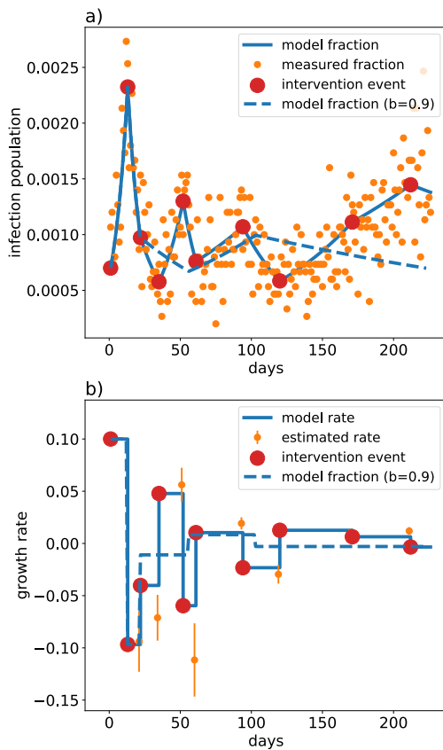
FIG. 3. Our algorithm implements policy releases and restrictions aiming at maintaining a vanishing growth rate. It intervenes whenever the estimated slope of the fraction of infected people is found to be non-zero, here with confidence level \alpha = 3 . We plot the model infection fraction U(t)/N and the detected infection fraction i(t) as a function of days in panel (a). The model growth rate k(t) (solid line) and the estimated growth rate k_{\text{est}} at times of intervention are shown in panel (b) for the parameters i(0) = 0.0012 , k_1 = 0.1 , and a test rate of r = 15'000 \text{ day}^{-1} . The dashed blue line corresponds to a history of interventions where we assumed that the effect of policy interventions is better known (described by an uncertainty parameter b = 0.9 , instead of b = 0.5 ), so that convergence is much faster.
