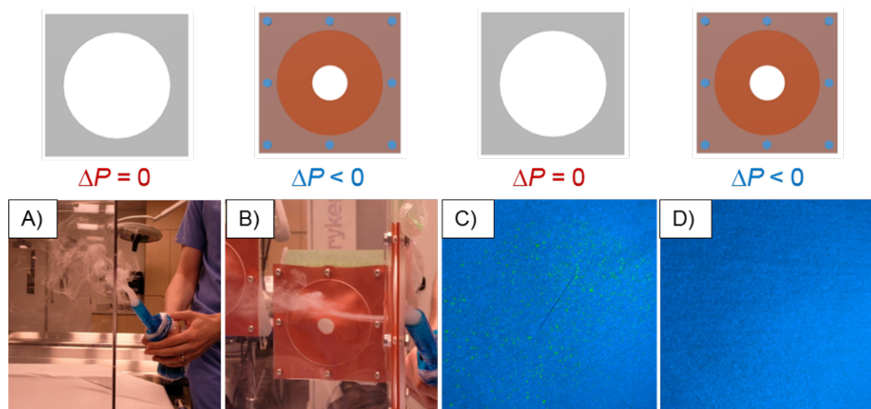
Figure 4. Photos depicting smoke entering enclosures with A) open ports under ambient pressure and B) ACE ports under negative pressure with schematic illustrations (top). Photos depicting fluorescein spatter on filter paper through C) open ports under ambient pressure and D) ACE ports under negative pressure.
