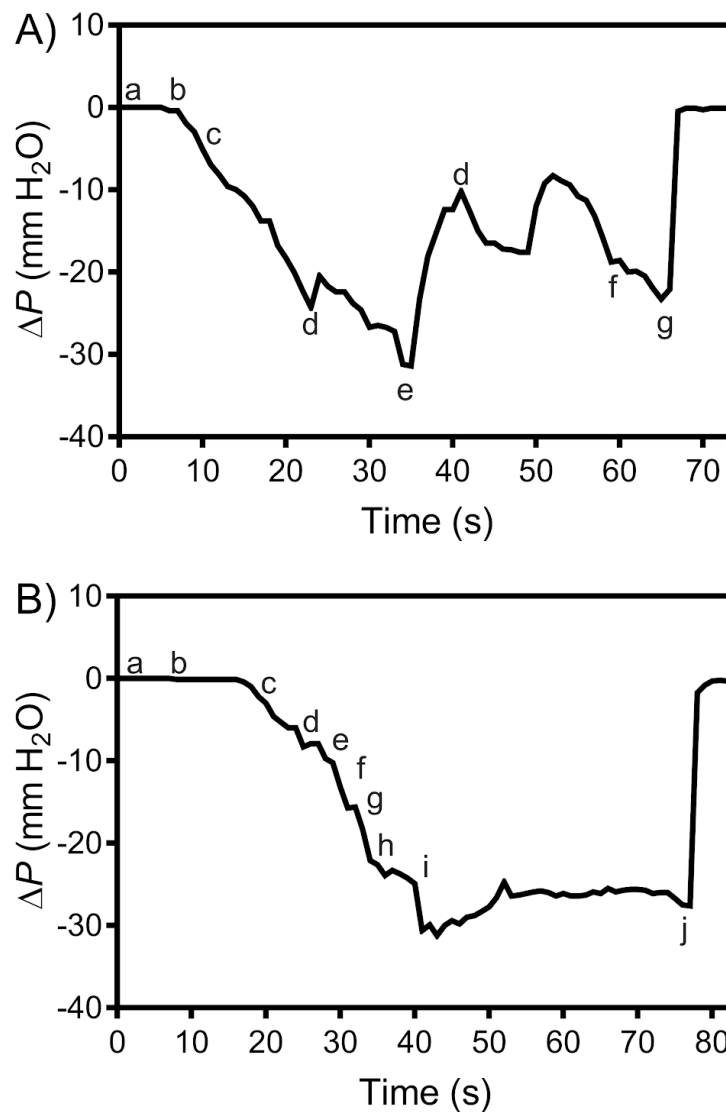
Figure 3. A) Differential pressure during simulated manual ventilation within the ACE with BVM at 15 L min -1 O 2 . a: Operator's hands enter ACE ports. b: BVM applied to the simulated patient. c: Manual ventilation
