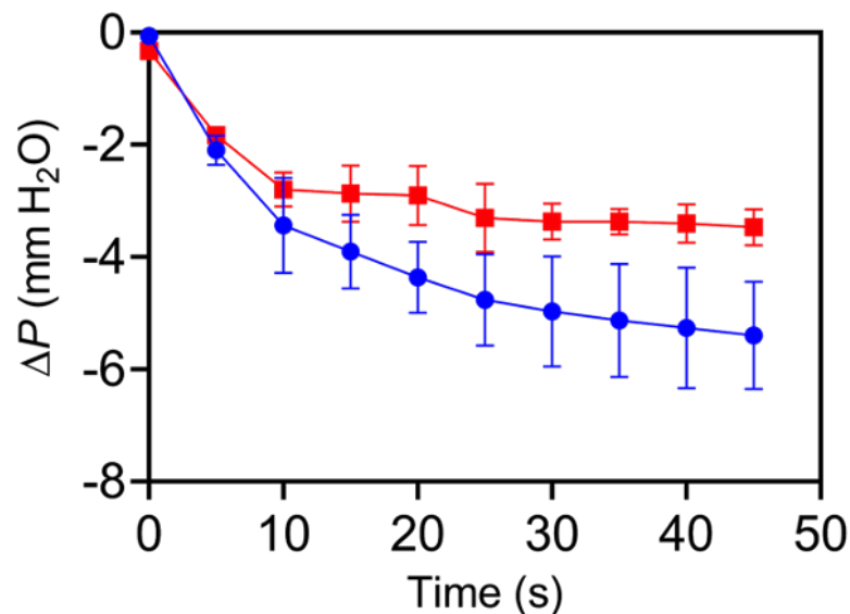
Figure 2. Differential pressure with front ports in use when: (red) side ports are covered with plastic sheets and (blue) a second user places his/her arms in the side ports (both users wearing recommended PPE for AGMPs). Plots are averages of three trials, with error bars indicating standard deviation.
