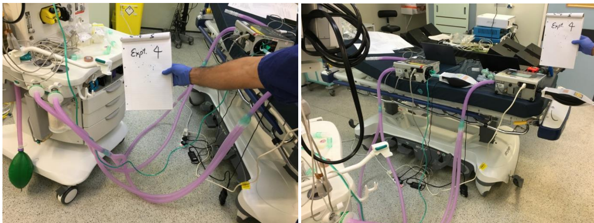
Figure 3. Dual-test lung ventilation system with two Fluke Gas Flow Analysers
