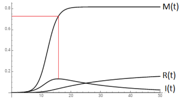
FIG. 2. SIMR model epidemic development ( m=0.2, \beta=0.6, \gamma=0.05 ).
