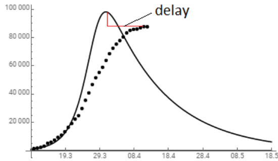
FIG. 5. Comparison of the dynamics of the number of cases during the COVID-19 epidemic in Spain according to the SIMR model (solid line) with statistical data [3] (dots). The SIMR parameters are taken as m=0.39 , \beta=0.52 , \gamma=0.06 .
