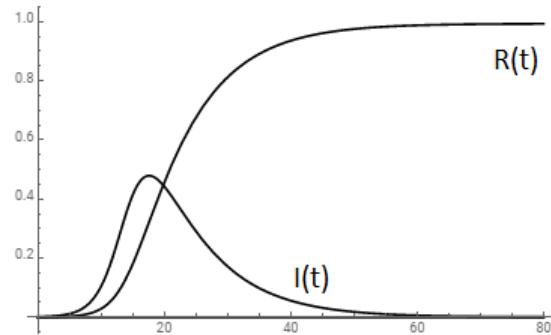
FIG. 1. SIR model epidemic development ( \beta=0.6 , \gamma=0.12 ).
