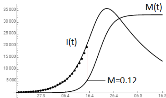
FIG. 7. Comparison of the dynamics of the number of cases during the COVID-19 epidemic in Russia according to the SIMR model (solid line) with statistical data [3] (dots). The SIMR parameters are taken as m=0.39 , \beta=0.35 , \gamma=0.05 .
