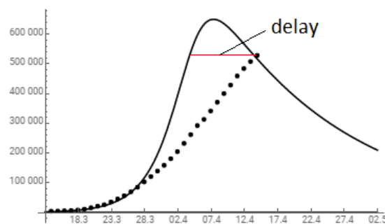
FIG. 8. Comparison of the dynamics of the number of cases during the COVID-19 epidemic in USA according to the SIMR model (solid line) with statistical data [3] (dots). The SIMR parameters are taken as m=0.39 , \beta=0.53 , \gamma=0.05 .
