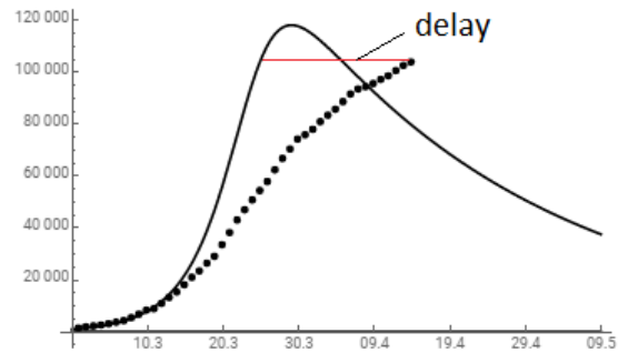
FIG. 4. Comparison of the dynamics of the number of cases during the COVID-19 epidemic in Italy according to the SIMR model (solid line) with statistical data [3] (dots). The SIMR parameters are taken as m=0.39 , \beta=0.39 , \gamma=0.03 .
