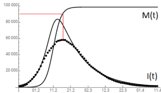
FIG. 3. Comparison of the dynamics of the number of cases during the COVID-19 epidemic in Wuhan (China) according to the SIMR model (solid line) with statistical data [3] (dots). The SIMR parameters are taken as m=0.39 , \beta=0.45 , \gamma=0.071 . Here and in all further figures, the line I(t) shows the number of cases, and the line M(t) is normalized to saturation with the value of M = 1 (100% hidden immunization). The red line indicates the hidden immunization M = 0.9 at the peak of I(t) .
