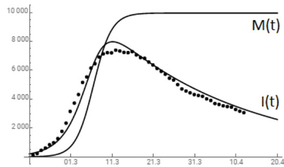
FIG. 9. Comparison of the dynamics of the number of cases during the COVID-19 epidemic in South Korea according to the SIMR model (solid line) with statistical data [3] (dots). The SIMR parameters are taken as m=0.39 , \beta=0.46 , \gamma=0.03 . Saturation of M(t) corresponds to 100% hidden immunization. Fraction of the mutated virus in the total initial infection is taken to be f=0.9 .
