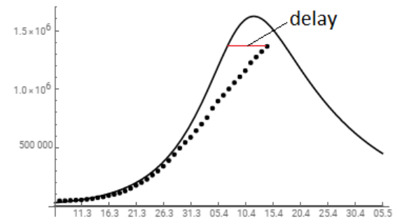
FIG. 10. Comparison of the dynamics of the number of cases during the COVID-19 epidemic in the world according to the SIMR model (solid line) with statistical data [3] (dots). The SIMR parameters are taken as m=0.39 , \beta=0.32 , \gamma=0.065 .
