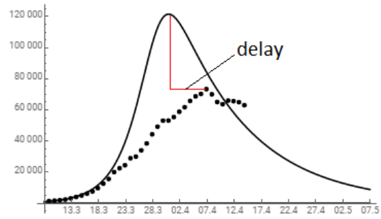
FIG. 6. Comparison of the dynamics of the number of cases during the COVID-19 epidemic in Germany according to the SIMR model (solid line) with statistical data [3] (dots). The SIMR parameters are taken as m=0.39 , \beta=0.53 , \gamma=0.075 .
