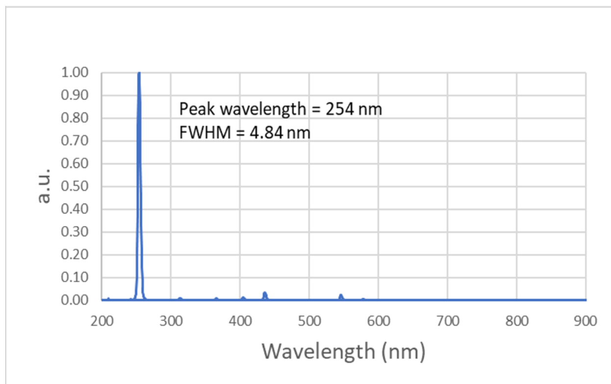
Figure 1: Spectrum of emission of the HNS 15 W G13 OSRAM luminaire.
