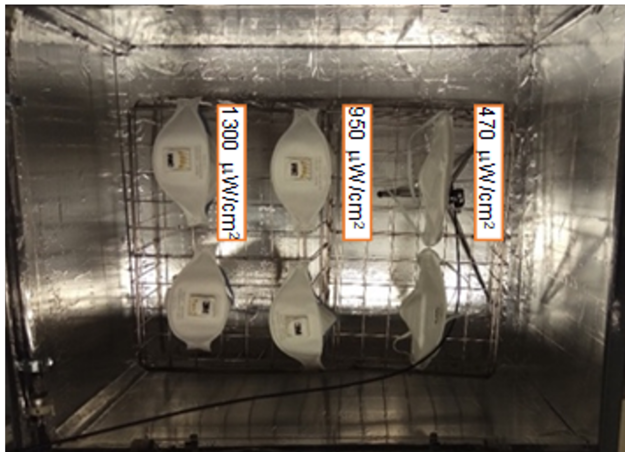
Figure 6: Photography of the opened UVGI irradiator with the respirator placed in the configuration of Figure 3c, indicating the irradiance received at three different positions.
