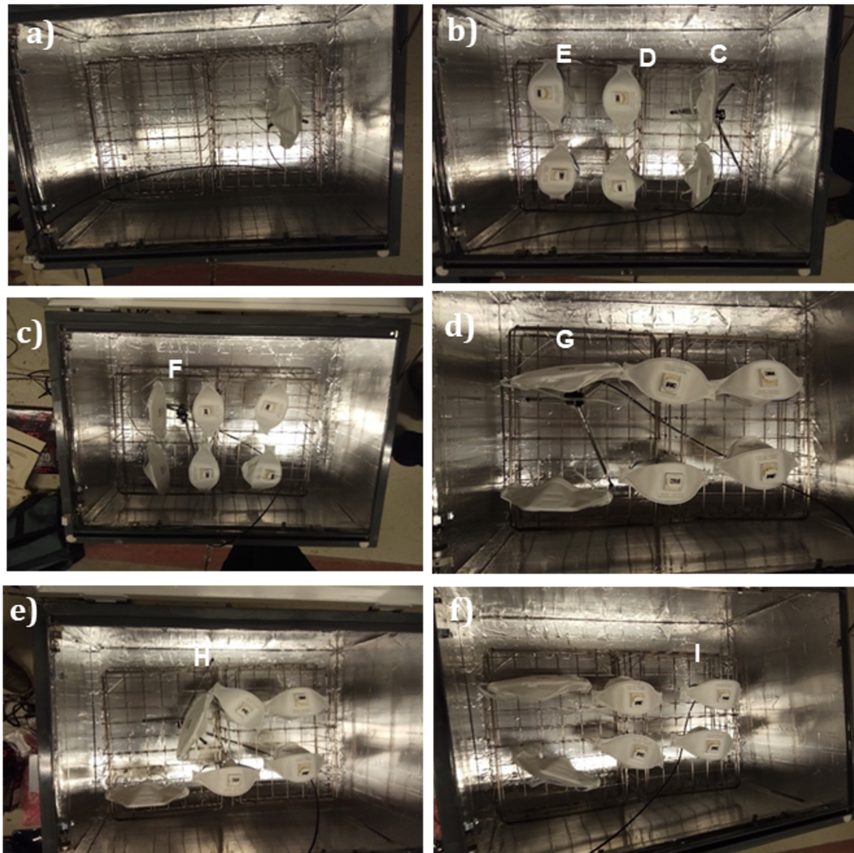
Figure 3: Photography of the inner part of the chamber, with the grating located at 16 cm from the luminaires plane a) detector just below the respirator, and 6 respirators placed in different configurations b) masks placed vertically with the shorter masks closer to the left lamp c) masks placed vertically with the taller masks closer to the left lamp d) masks placed horizontally, e) detector placed below one of the tall masks near the middle of the box; and f) detector placed below one of the short masks near the right side of the box, far from the lamp on the left side of the box.
