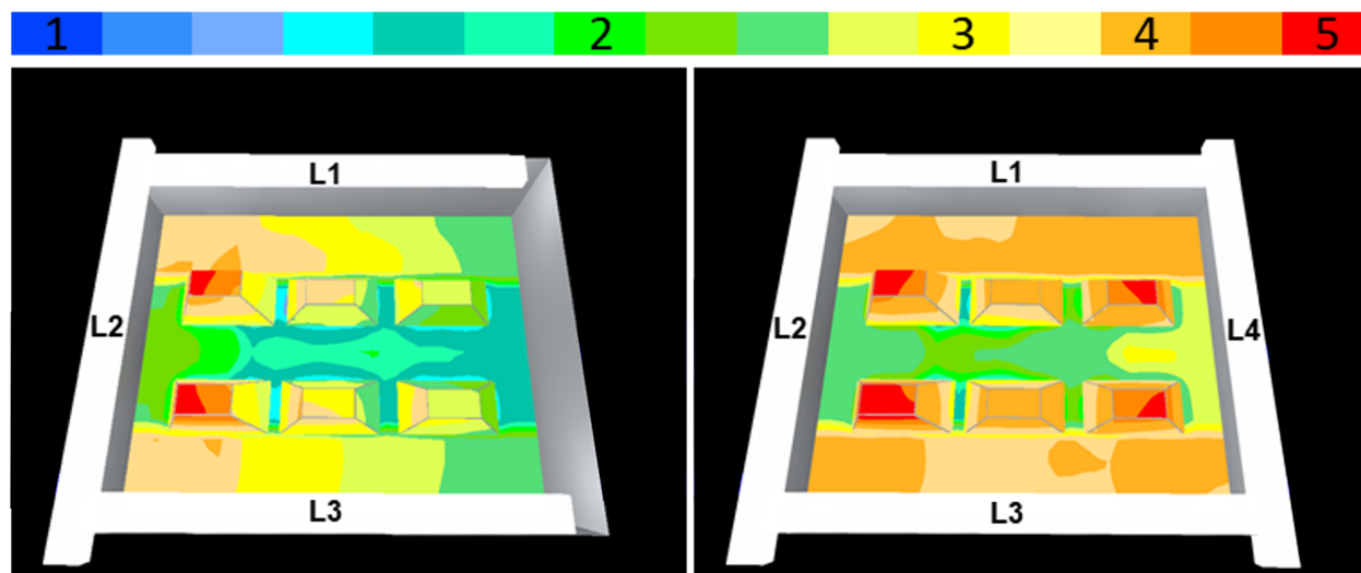
Figure 5: Pseudocolor map of light distribution obtained with three and four lamps for two models of facial respiratory masks, oriented parallel to the long side of the box.
