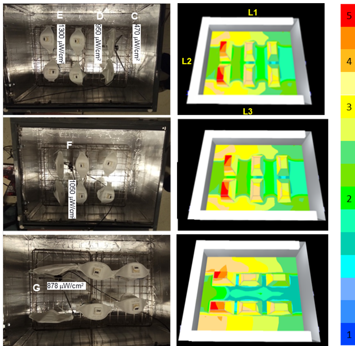
Figure 4: left) Representation of the experimental data obtained in the disinfection box; Right) simulated light distribution maps in pseudocolor maps inside the UVGI irradiator. The luminaires are marked in white and named L1, L2 and L3. Blue colors correspond to a reference amount of light. Green color represents a value equal to two times the reference value, yellow corresponds to three times, amber to four times, and red to 5 times.
