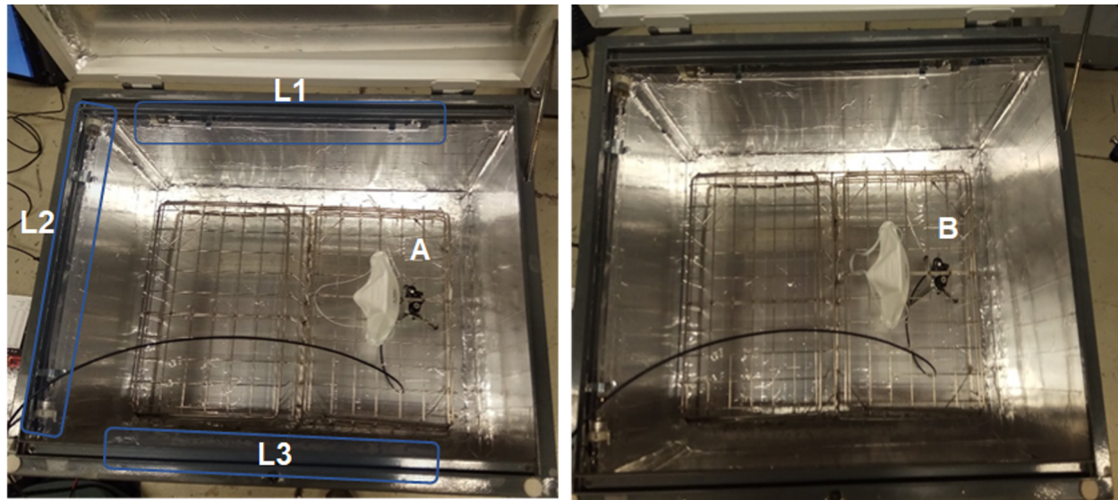
Figure 2: Photography of the inner part of the chamber, with the lamps L1 L2 and L3; the grating located at 10cm from the lamps plane; Position A, just beside the respirator; Position B, with the respirator placed 5 cm towards the left side.
